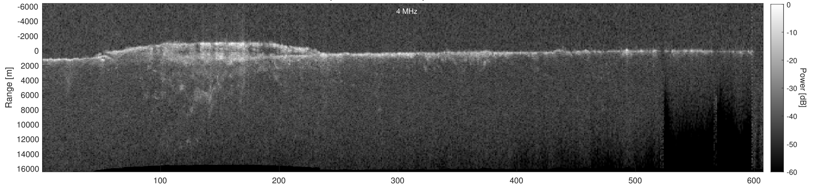
Orbit 7464, Depth-Corrected Cluttergram
