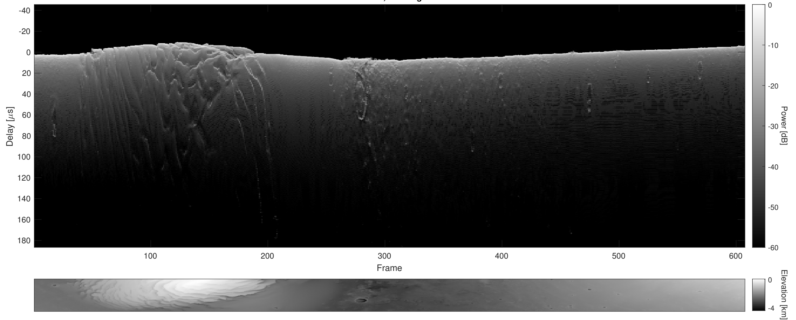
Orbit 7466, Cluttergram
