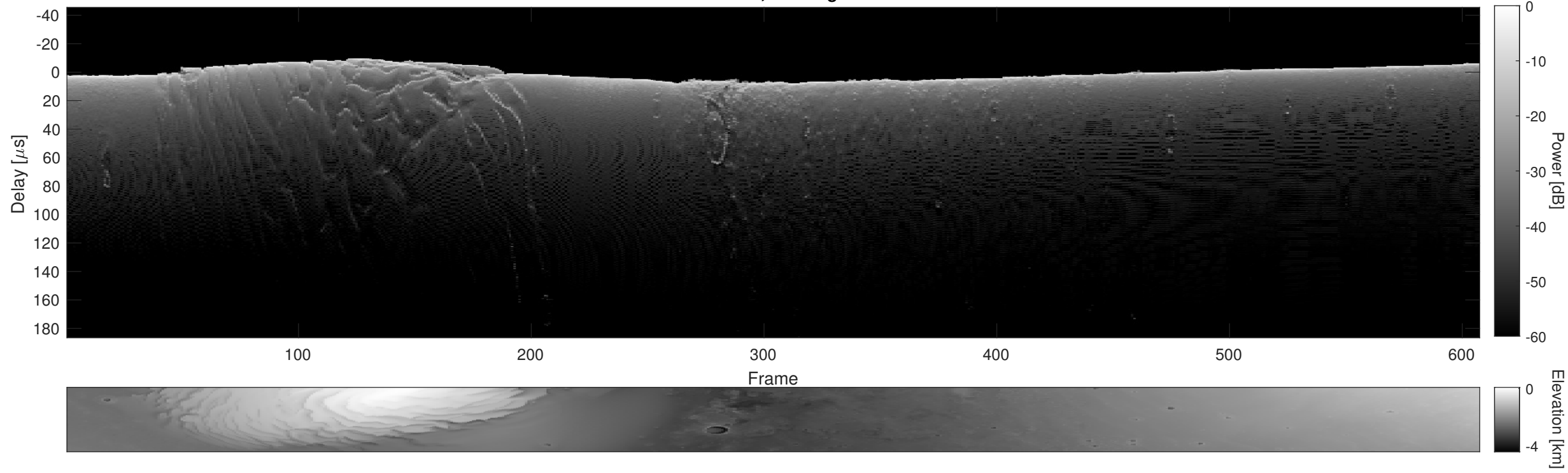
Orbit 7466, Cluttergram
