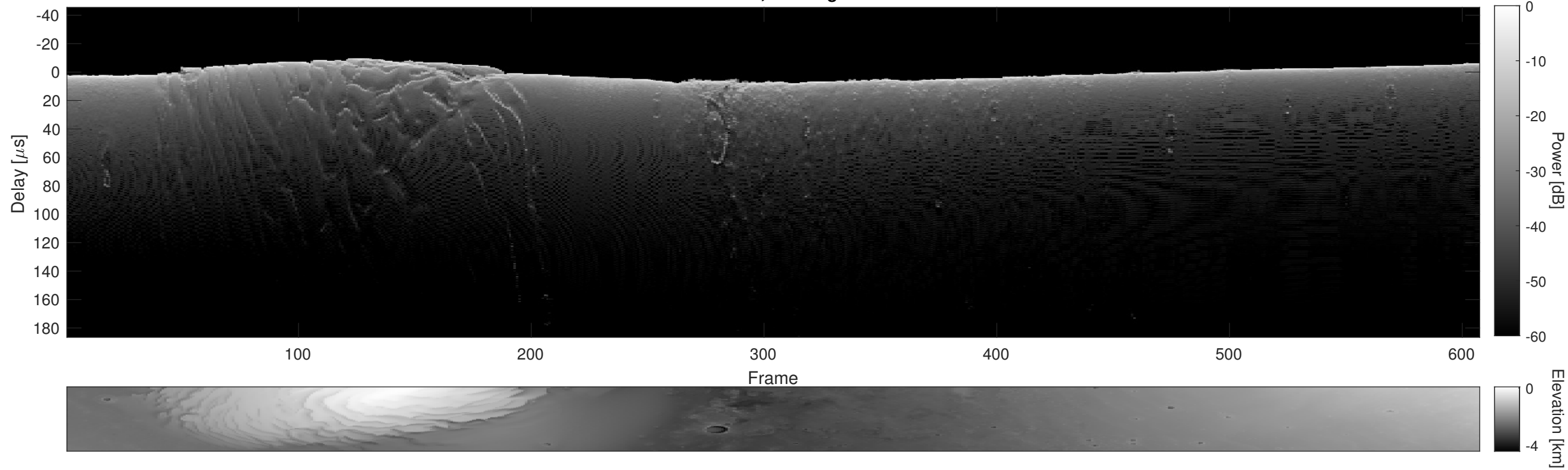
Orbit 7466, Cluttergram
