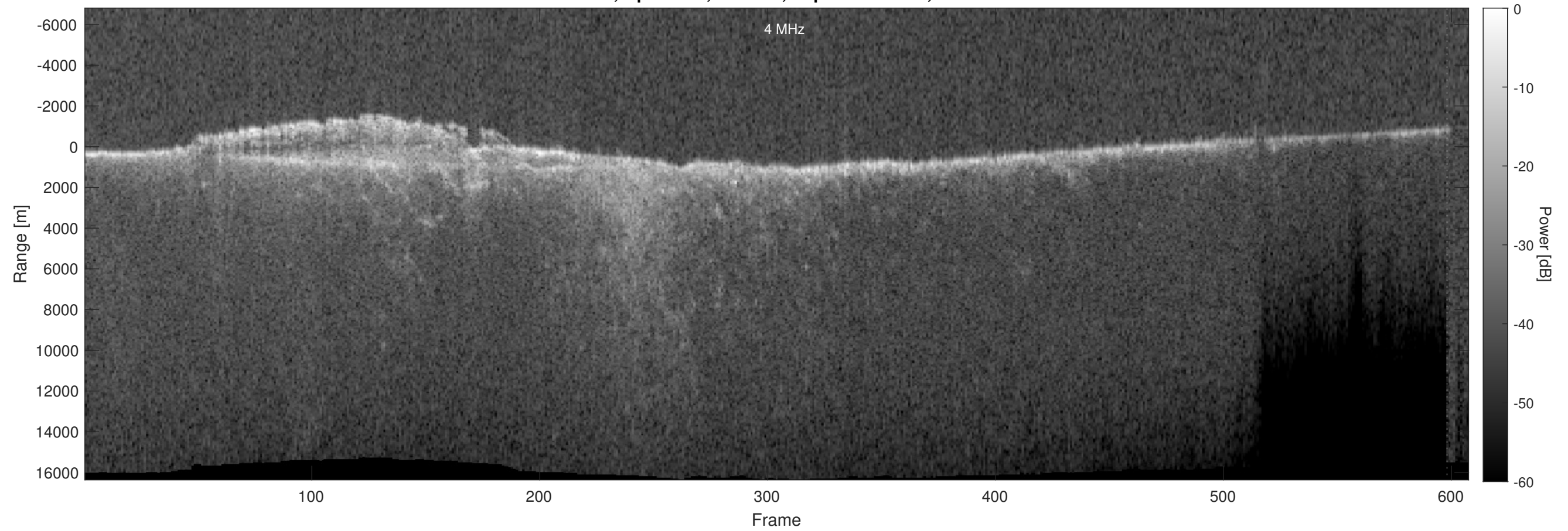
Orbit 7466, Optimized, Window, Depth-Corrected, Channel 2
