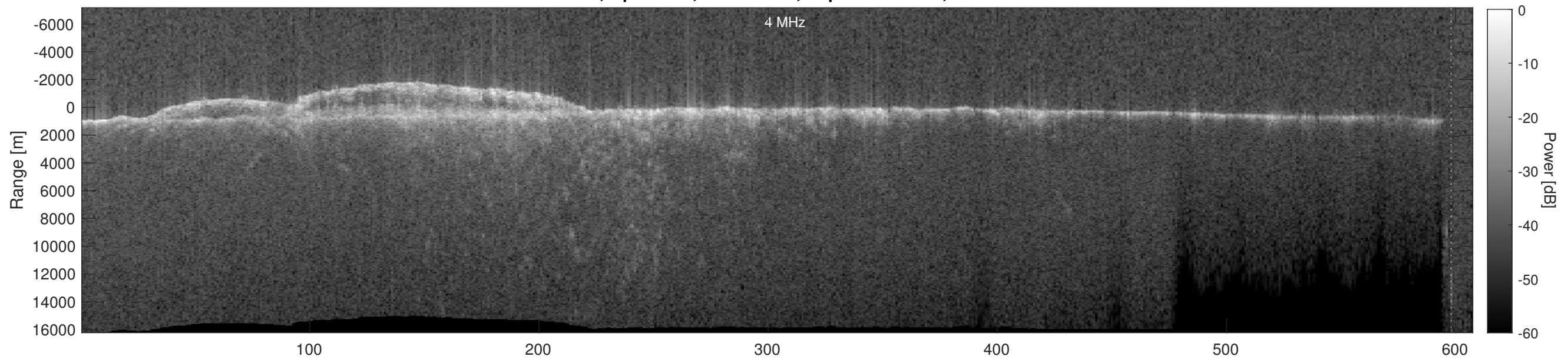
Orbit 7467, Depth-Corrected Cluttergram
