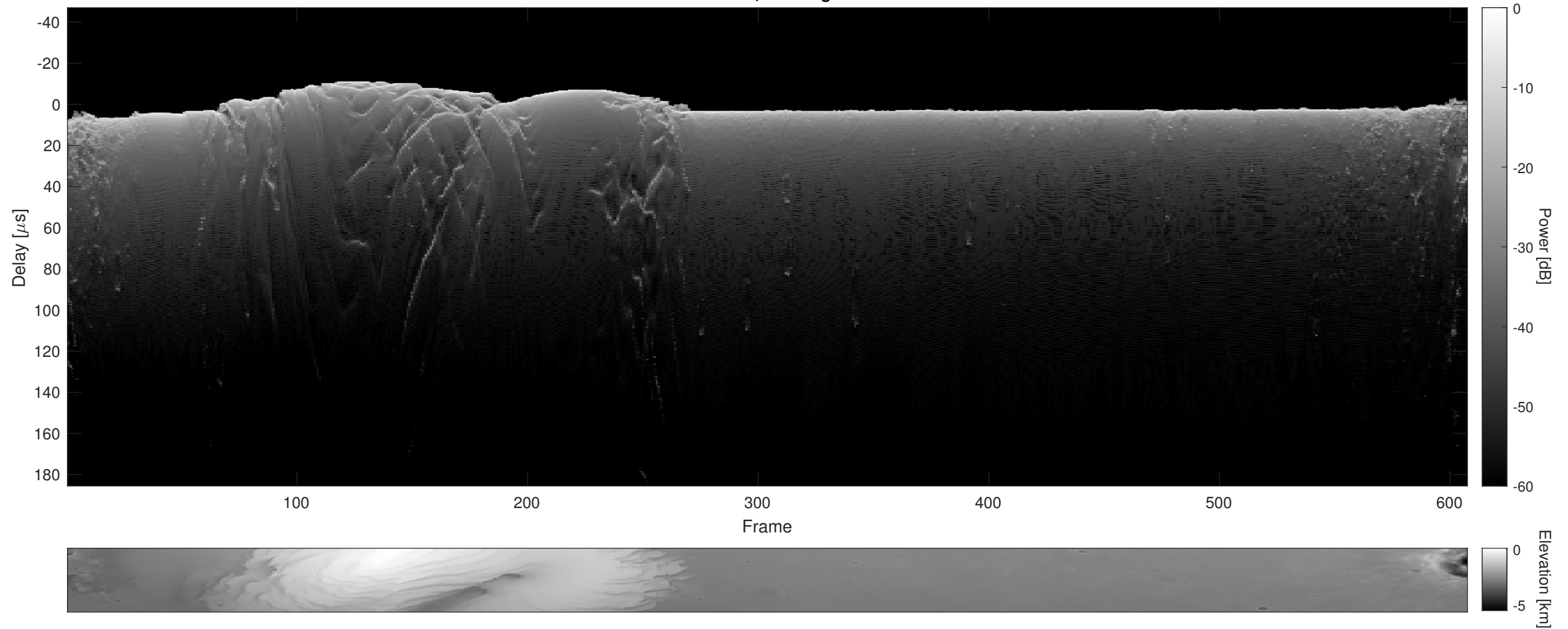
Orbit 7468, Cluttergram
