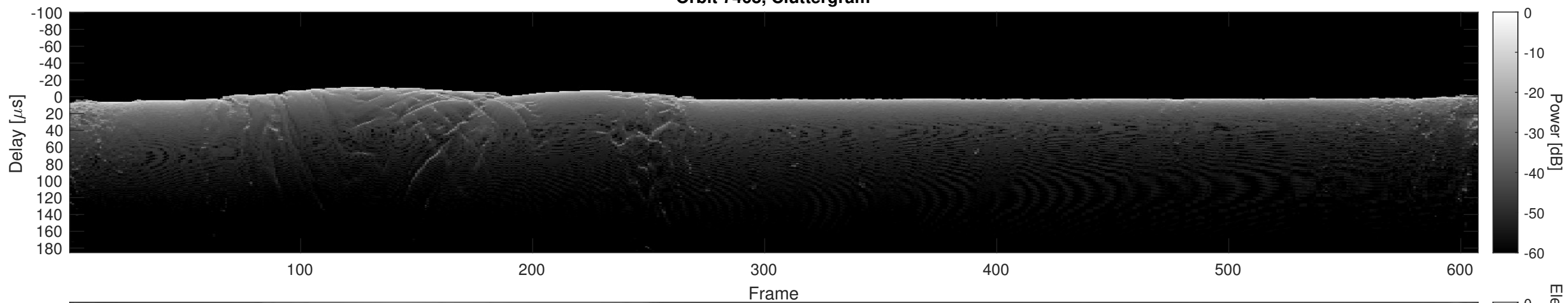
Orbit 7468, Cluttergram
