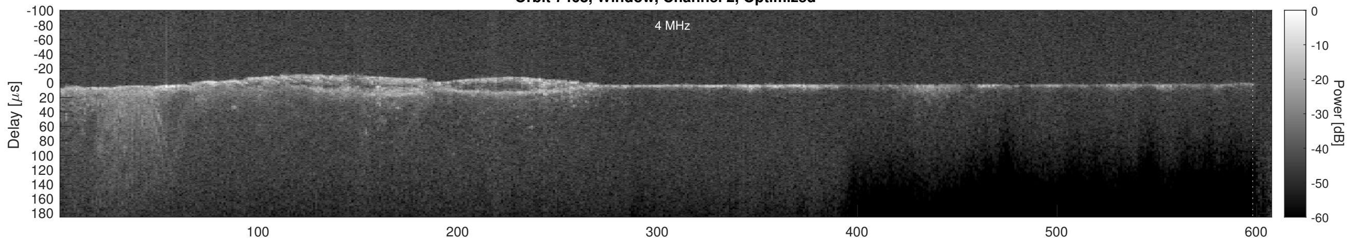
Orbit 7468, Cluttergram
