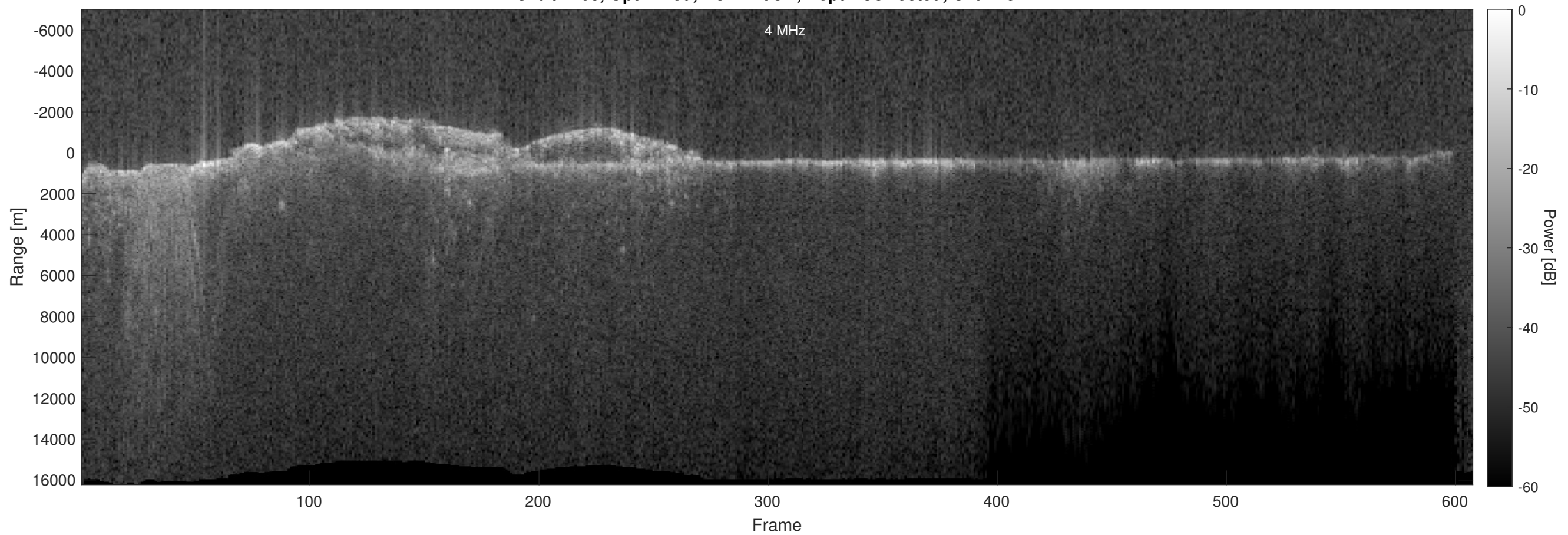
Orbit 7468, Optimized, No Window, Depth-Corrected, Channel 2
