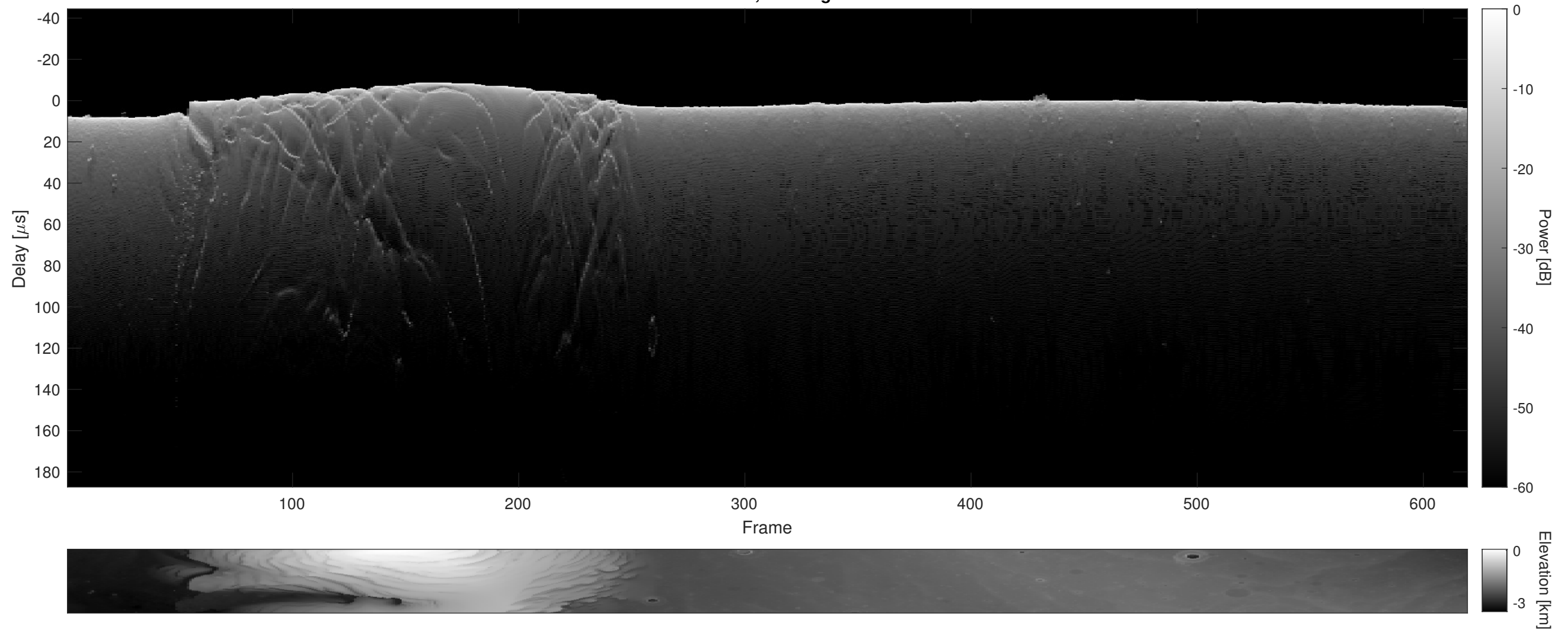
Orbit 7471, Cluttergram
