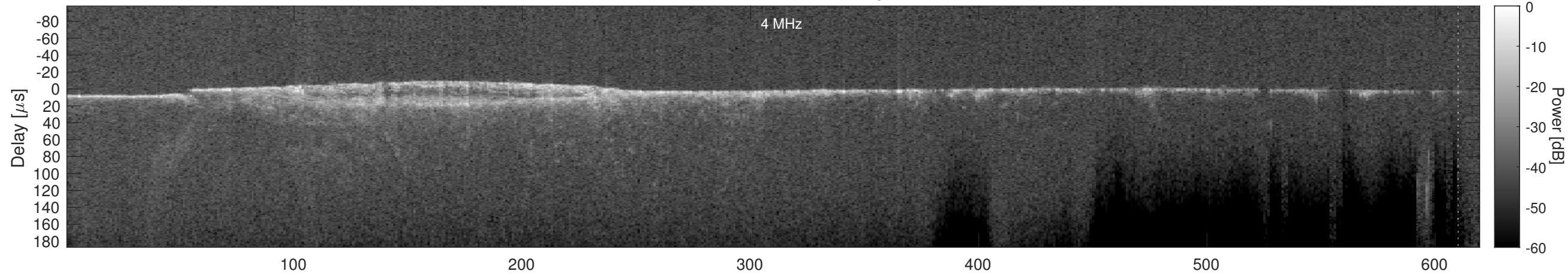
Orbit 7471, Cluttergram
