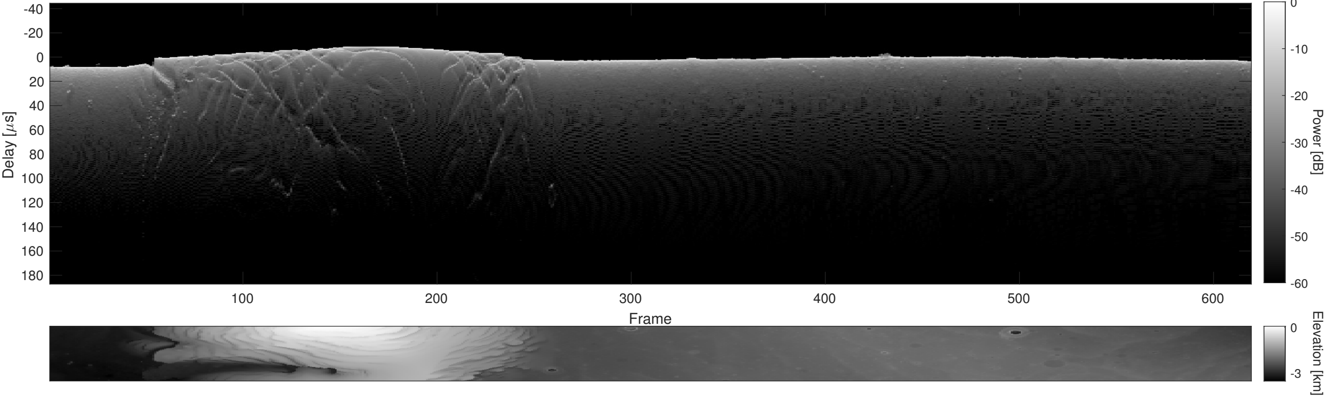
Orbit 7471, Cluttergram
