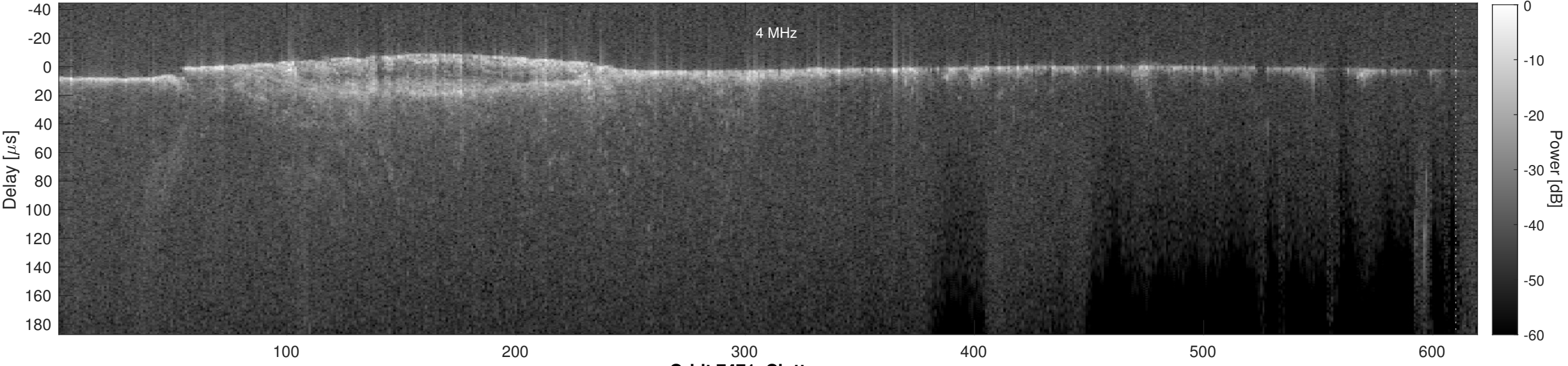
Orbit 7471, Cluttergram
