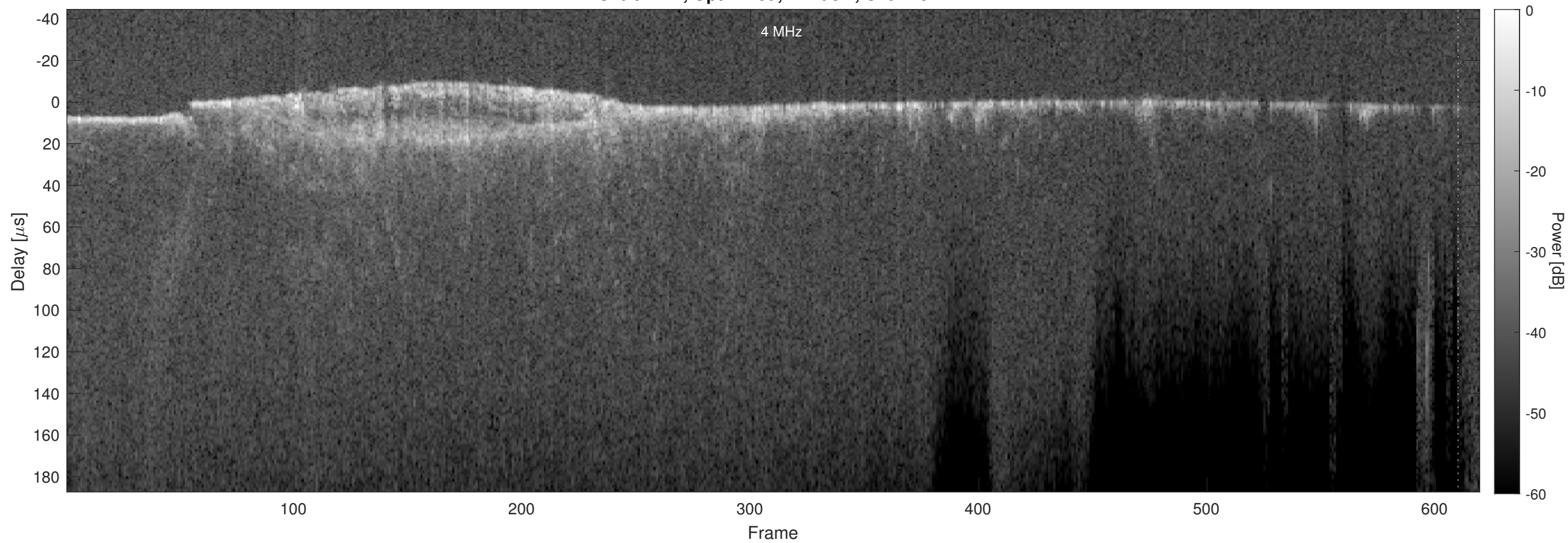
Orbit 7471, Optimized, Window, Channel 2
