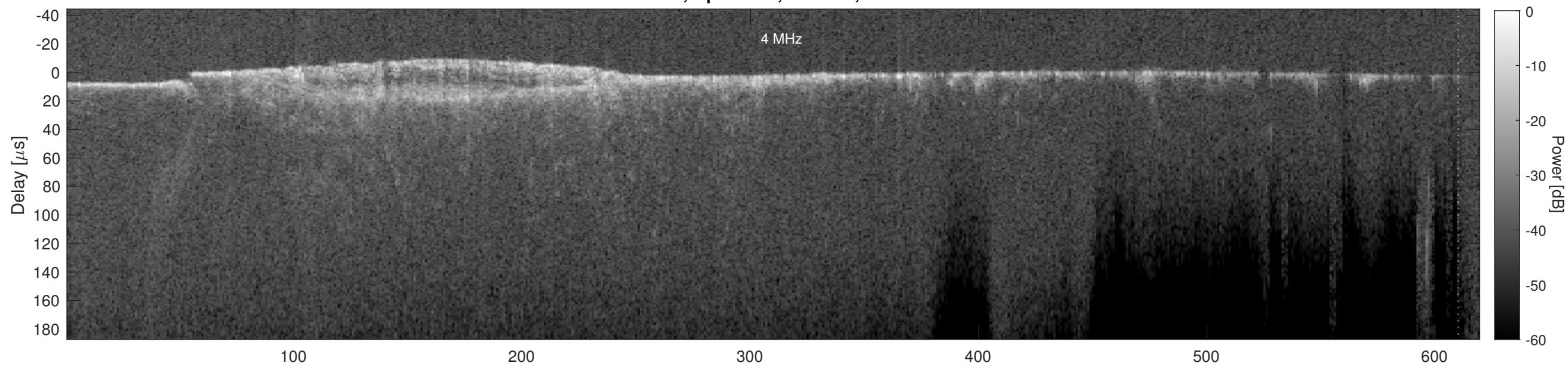
Orbit 7471, Cluttergram
