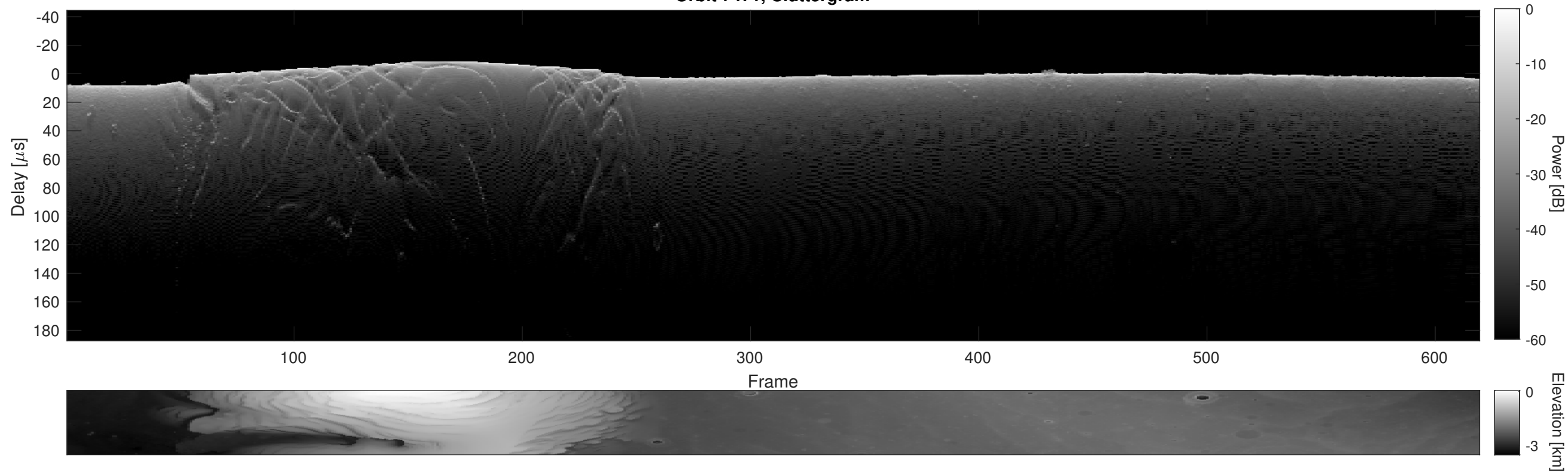
Orbit 7471, Cluttergram
