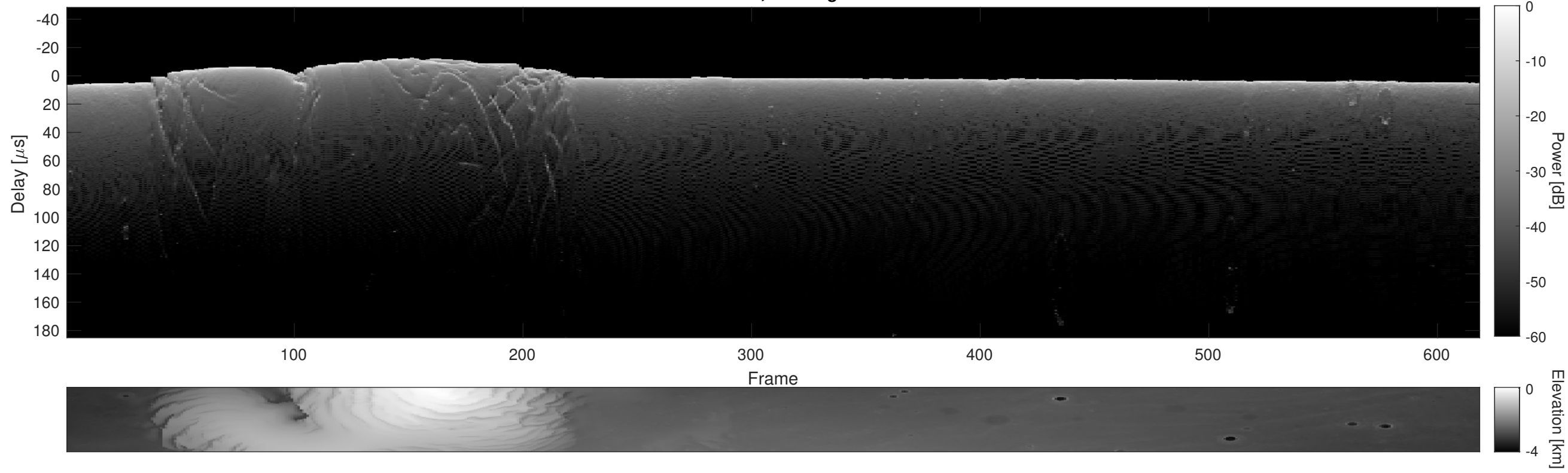
Orbit 7474, Cluttergram
