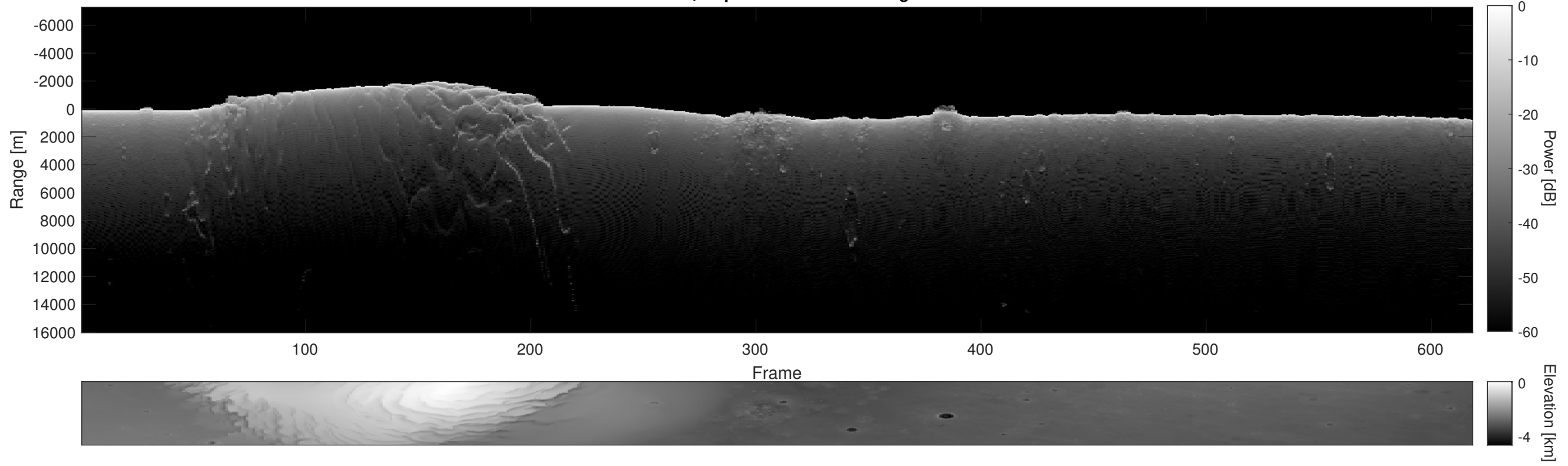
Orbit 7477, Depth-Corrected Cluttergram
