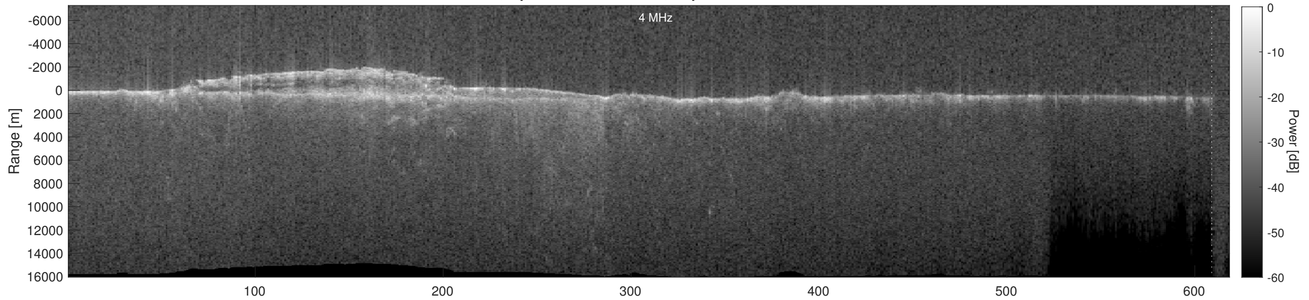
Orbit 7477, Depth-Corrected Cluttergram
