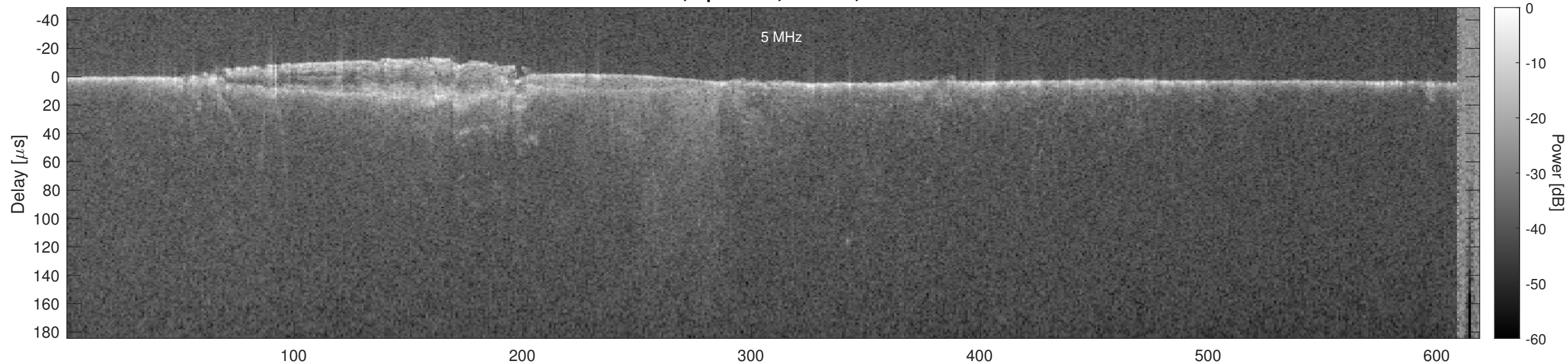
Orbit 7477, Optimized, Window, Channel 2
