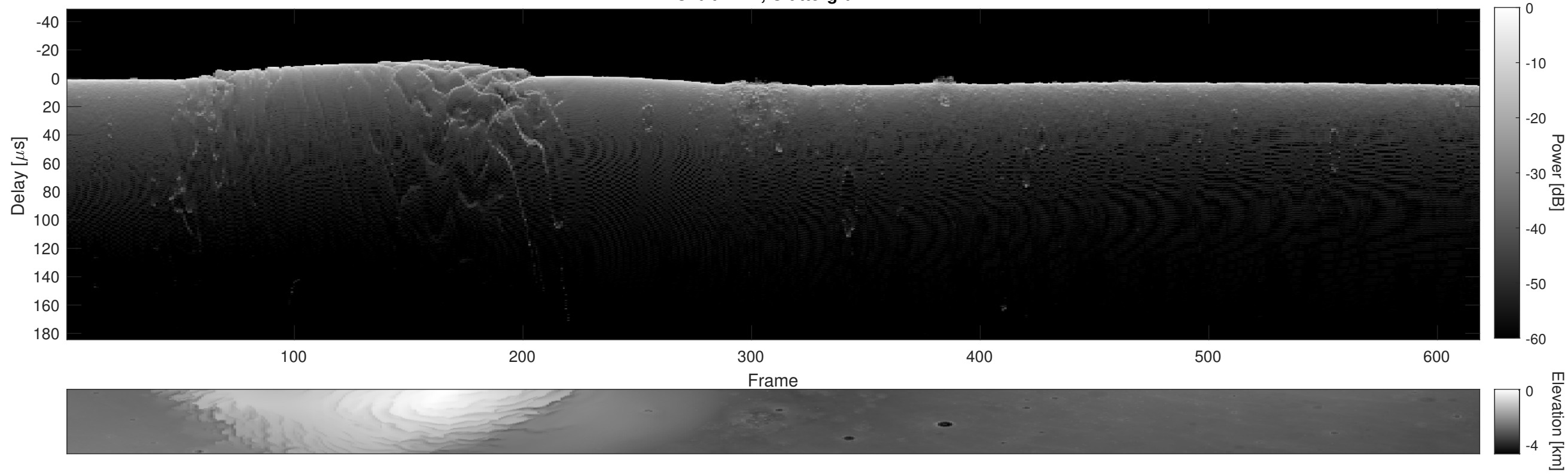
Orbit 7477, Cluttergram
