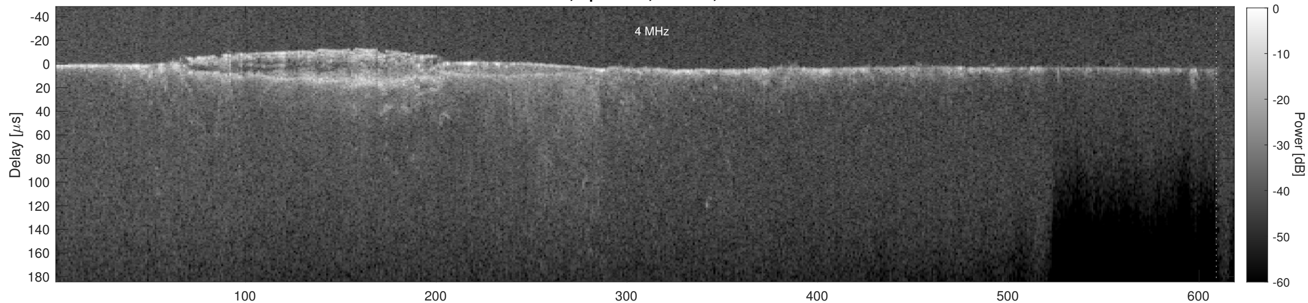
Orbit 7477, Cluttergram
