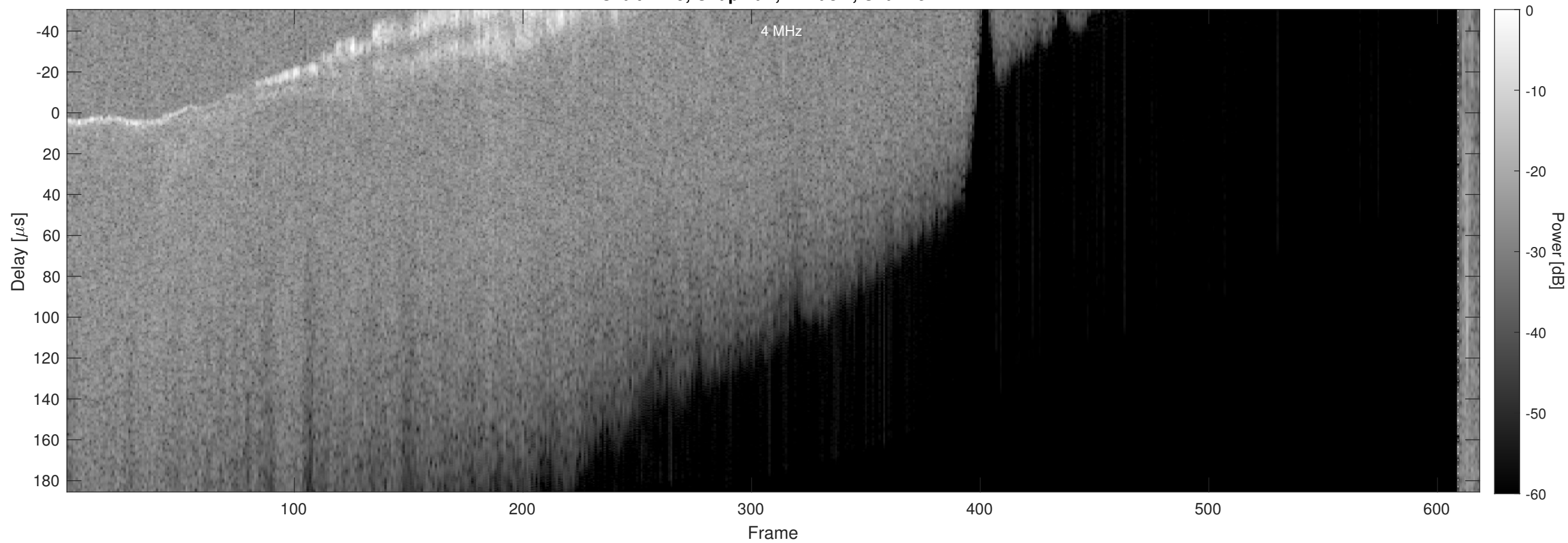
Orbit 7479, Chapman, Window, Channel 2
