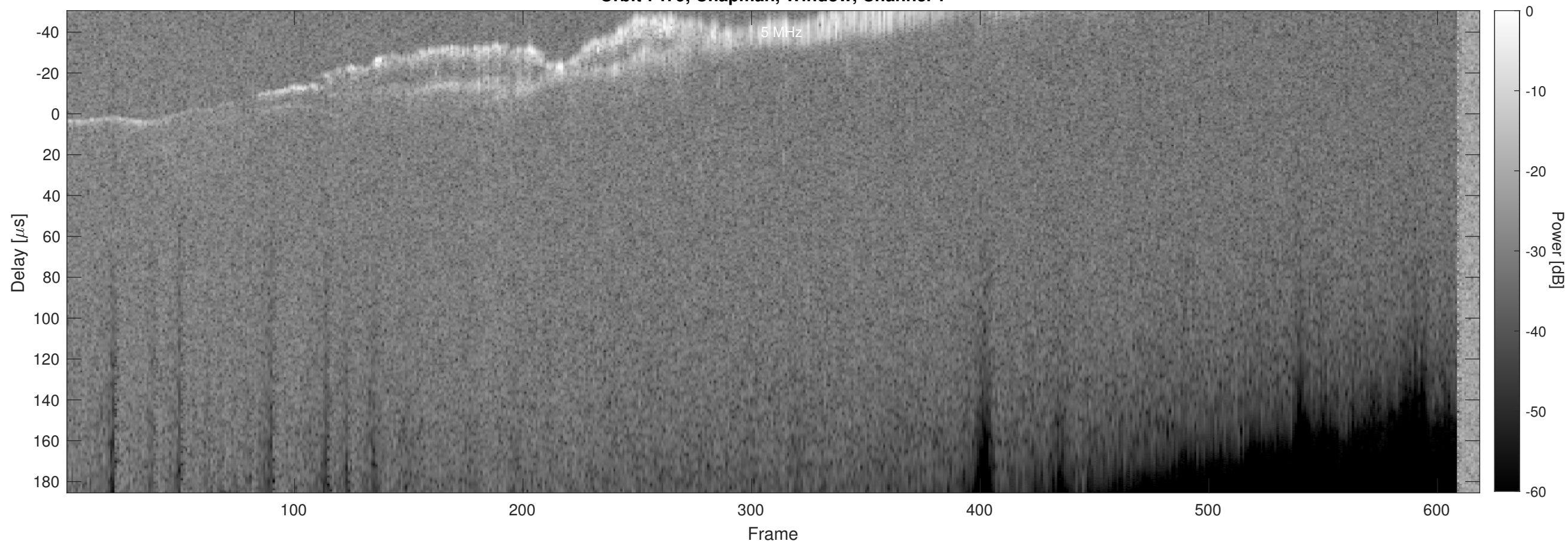
Orbit 7479, Chapman, Window, Channel 2
