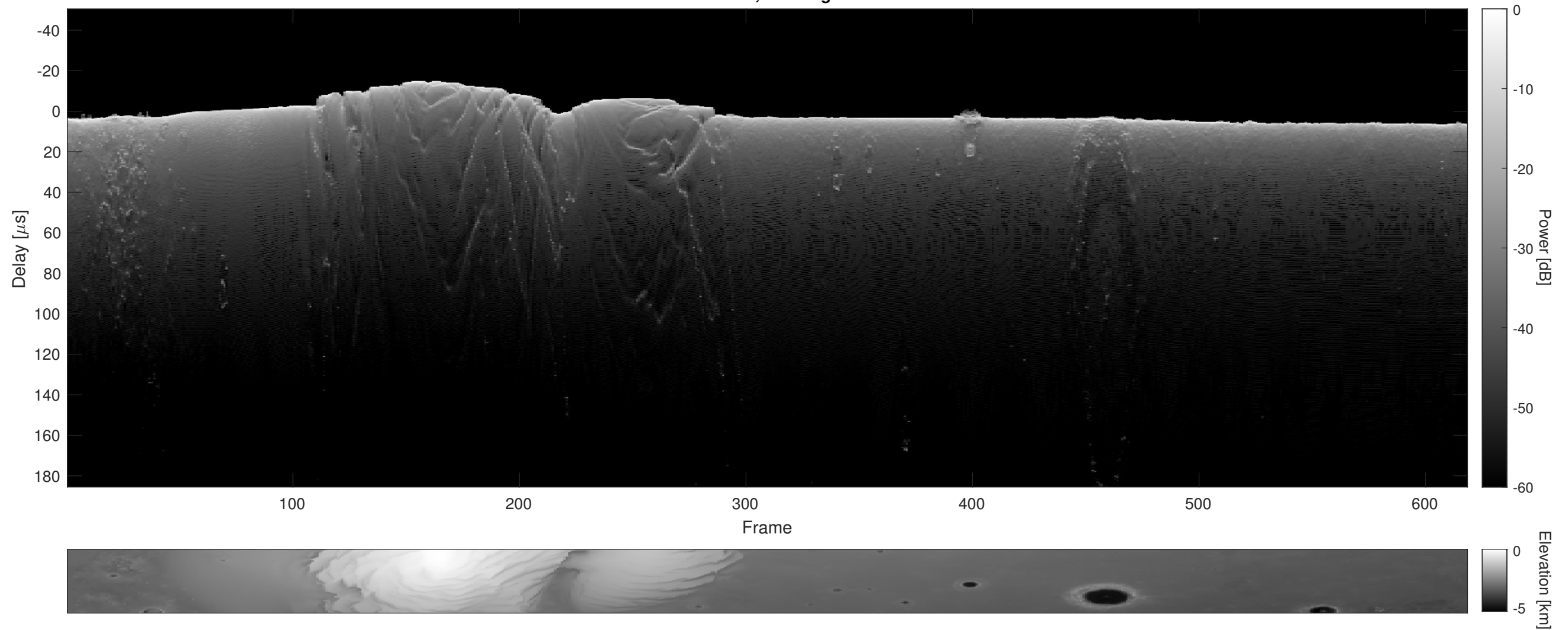
Orbit 7479, Cluttergram
