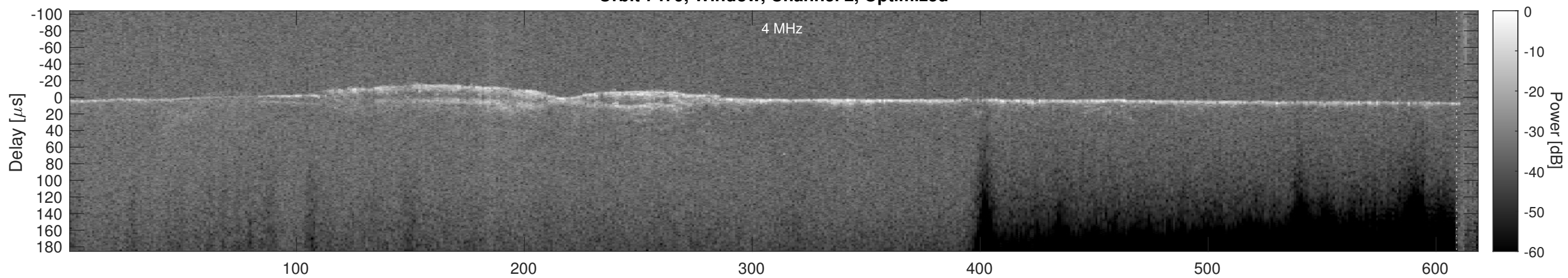
Orbit 7479, Cluttergram
