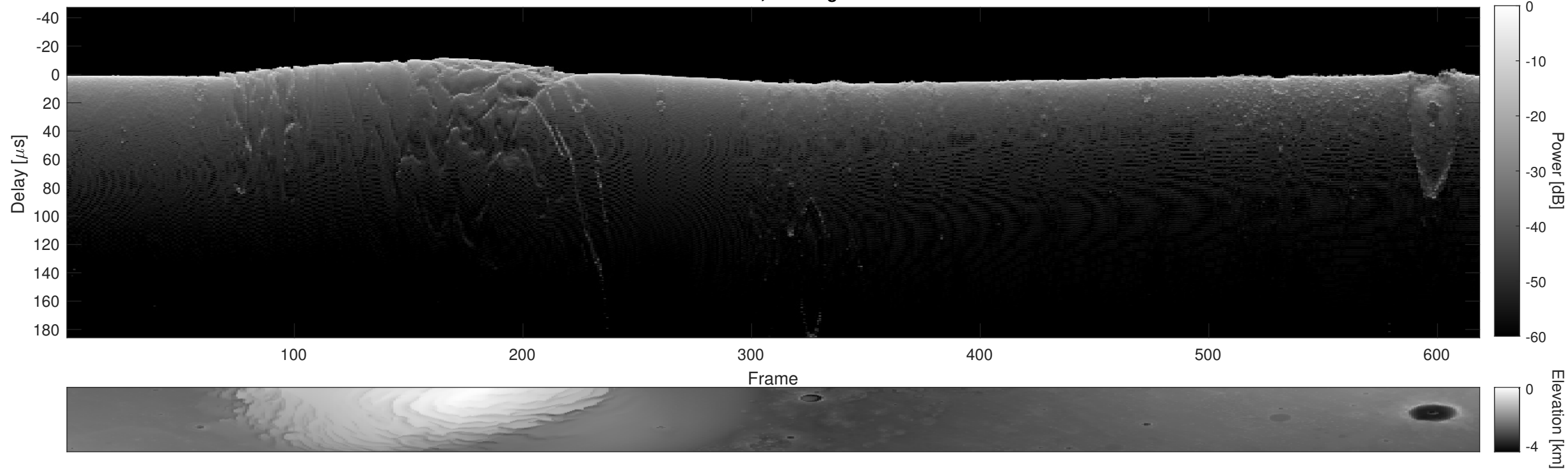
Orbit 7484, Cluttergram
