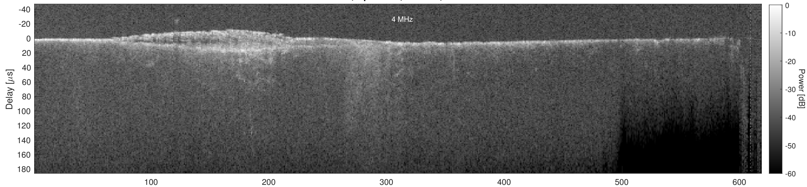
Orbit 7484, Cluttergram
