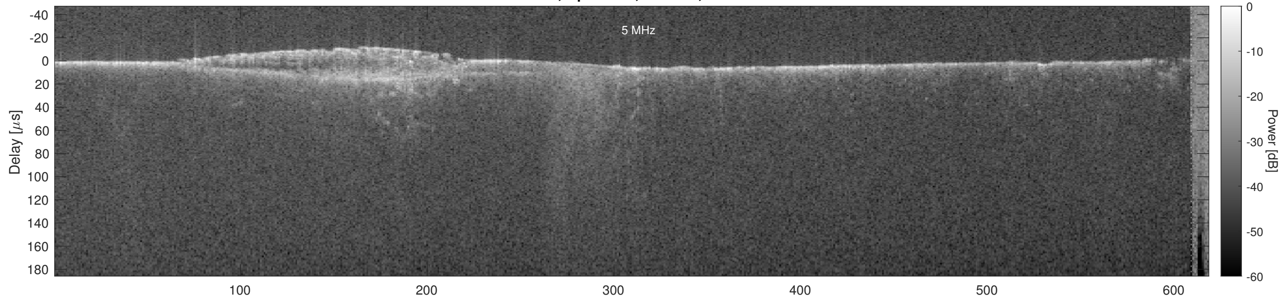
Orbit 7484, Optimized, Window, Channel 2
