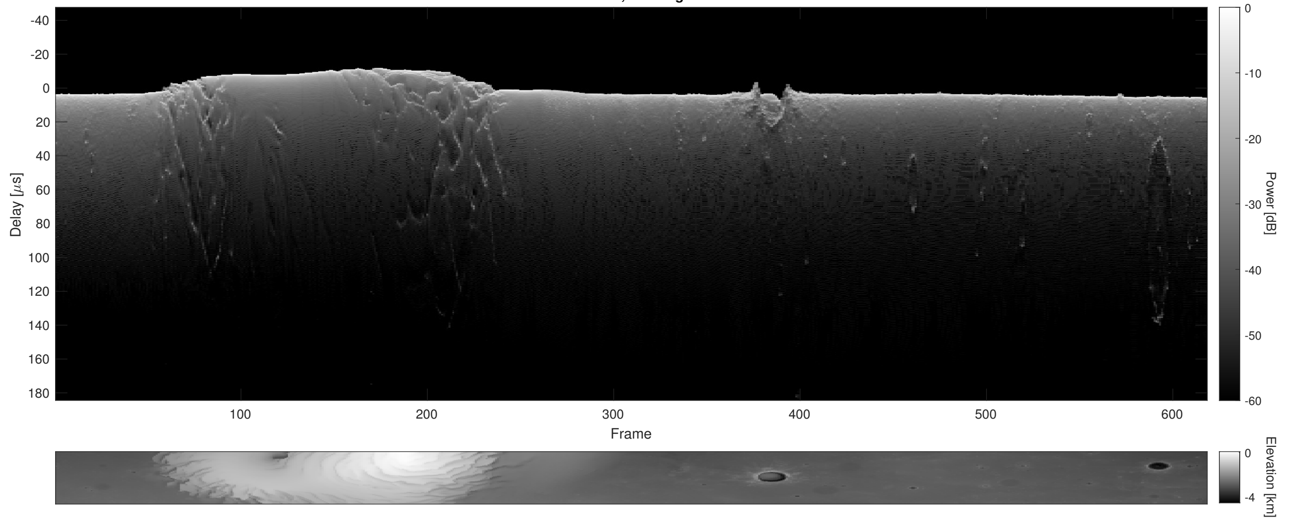
Orbit 7488, Cluttergram
