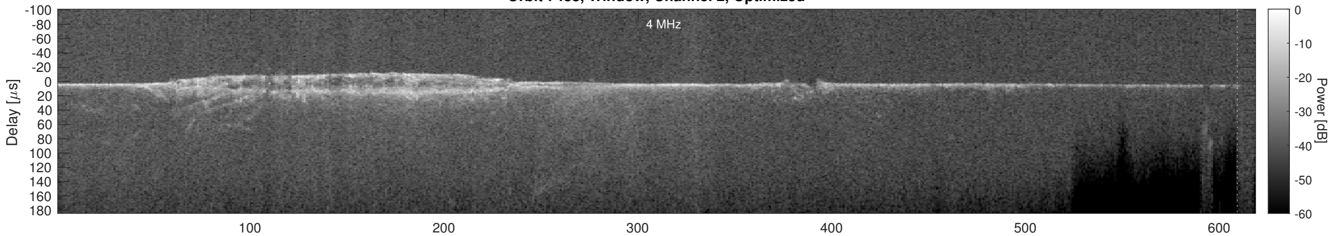
Orbit 7488, Cluttergram
