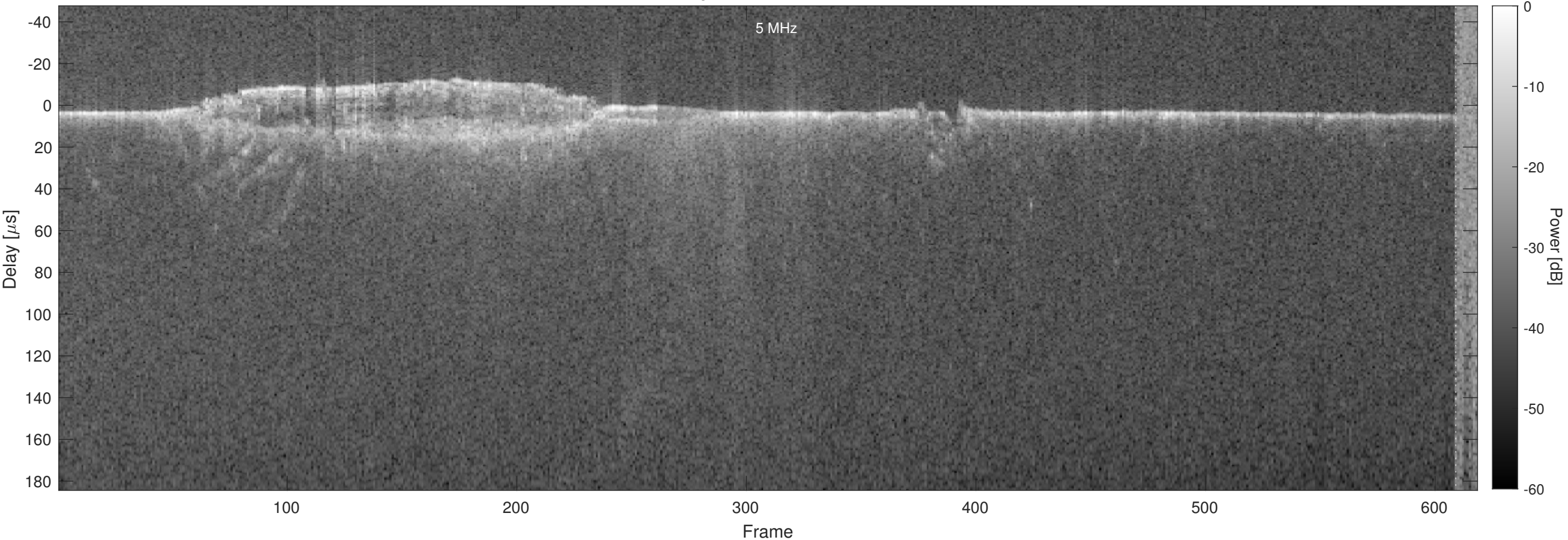
Orbit 7488, Optimized, Window, Channel 2
