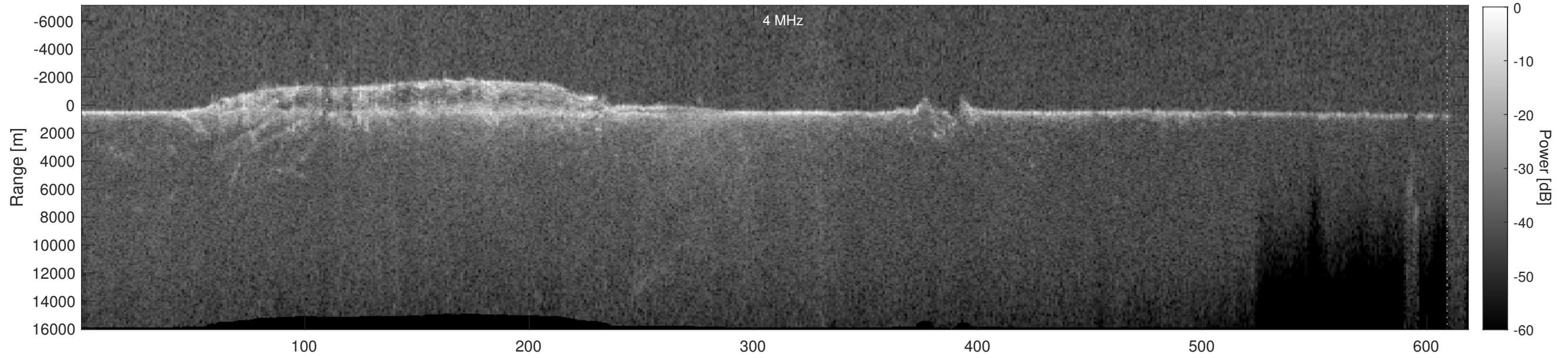
Orbit 7488, Depth-Corrected Cluttergram
