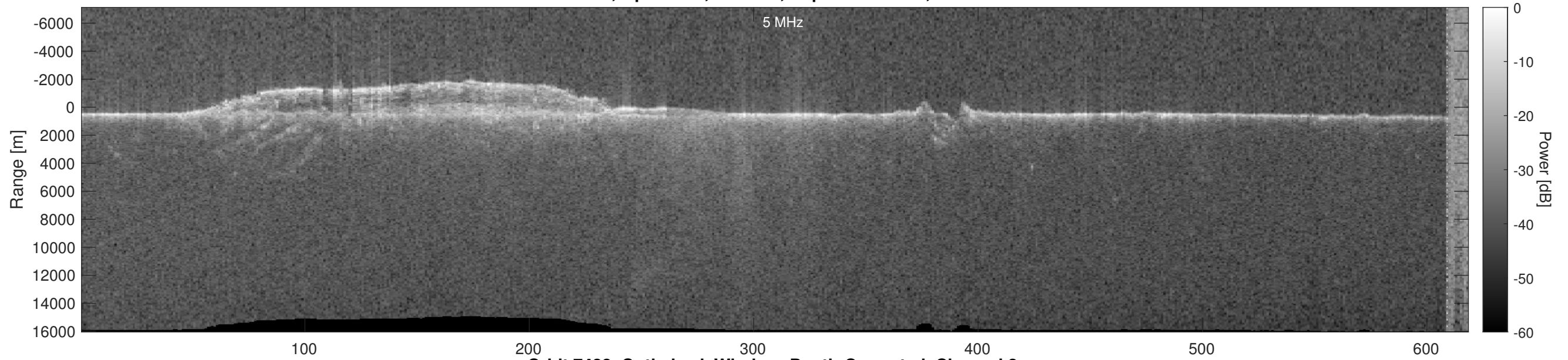
Orbit 7488, Optimized, Window, Depth-Corrected, Channel 2
