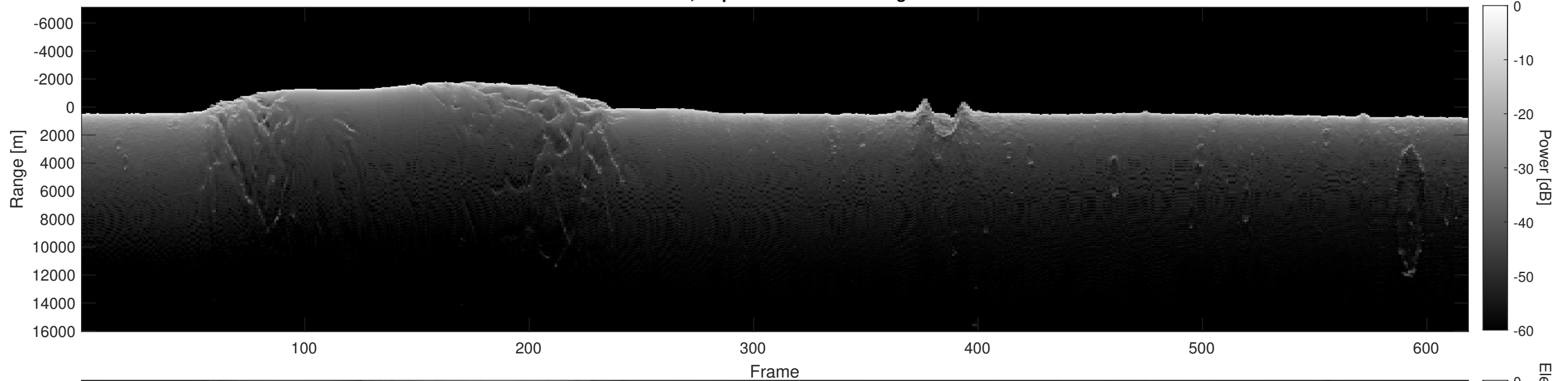
Orbit 7488, Depth-Corrected Cluttergram
