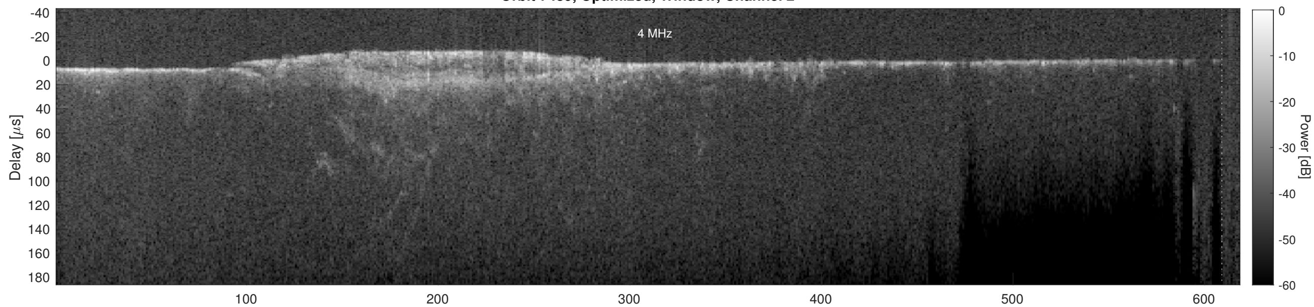
Orbit 7489, Cluttergram
