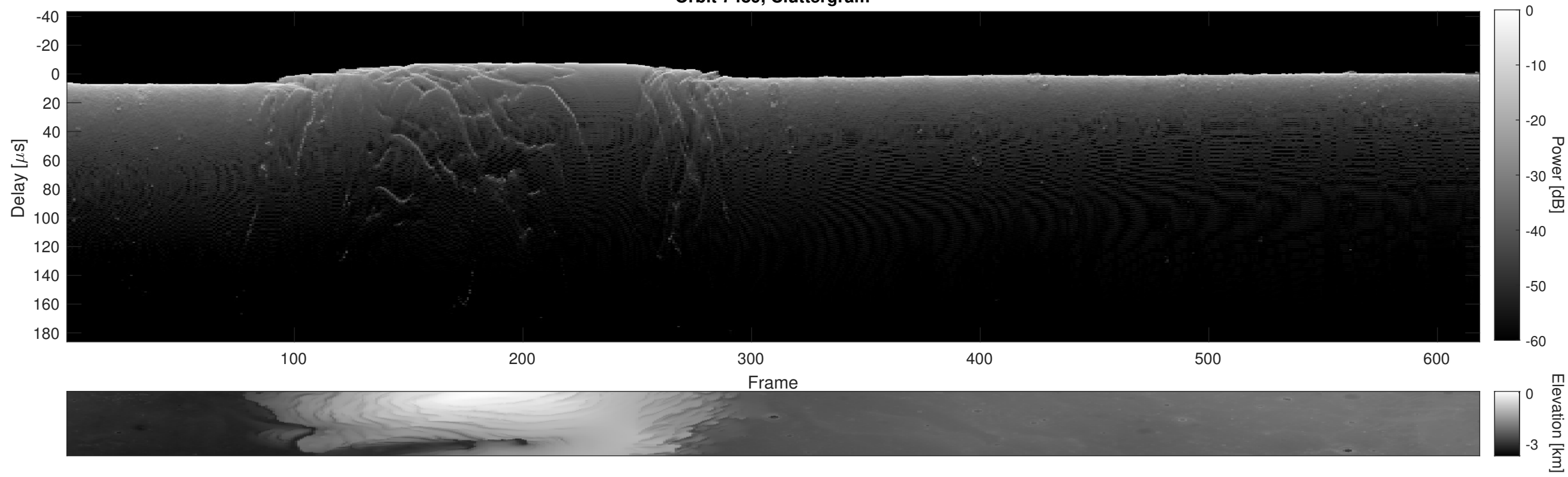
Orbit 7489, Cluttergram
