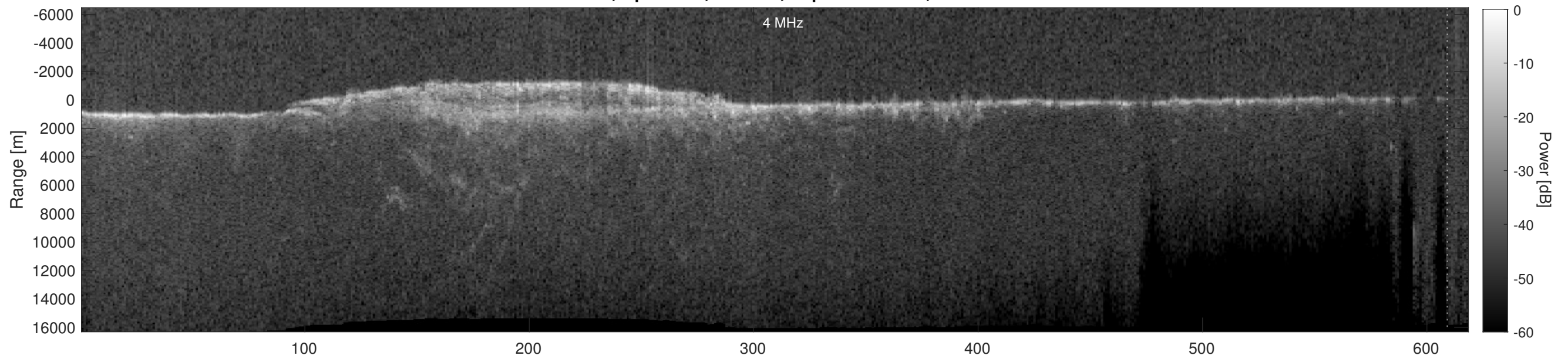
Orbit 7489, Depth-Corrected Cluttergram
