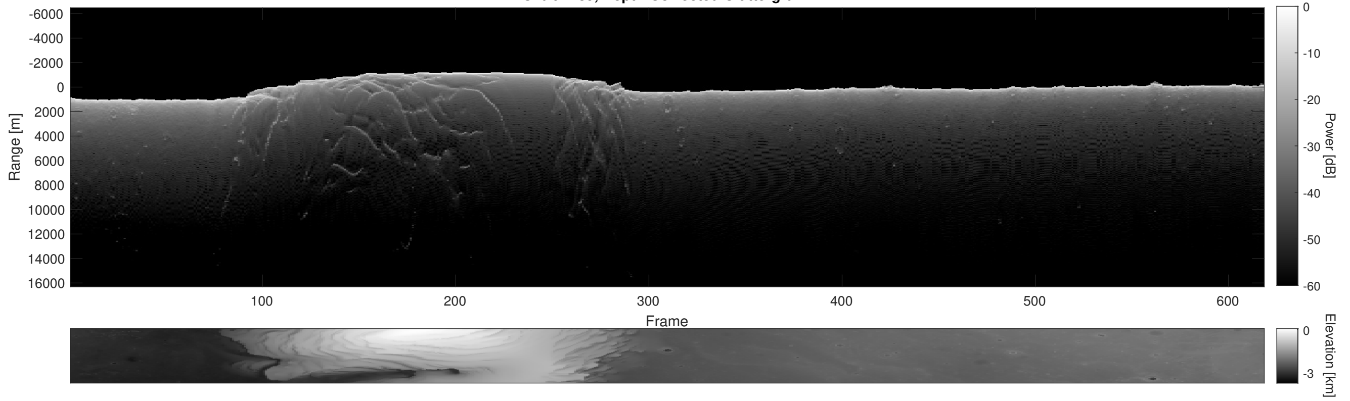
Orbit 7489, Depth-Corrected Cluttergram
