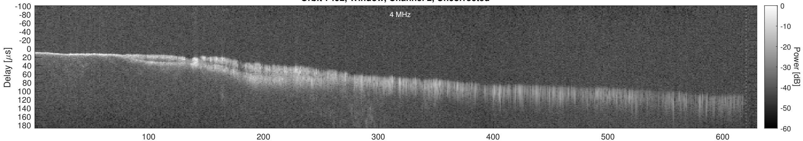
Orbit 7492, Window, Channel 2, Chapman
