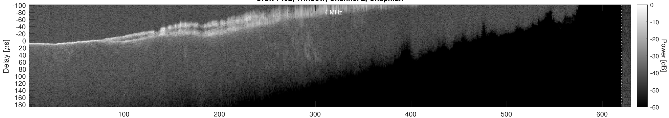
Orbit 7492, Window, Channel 2, Optimized
