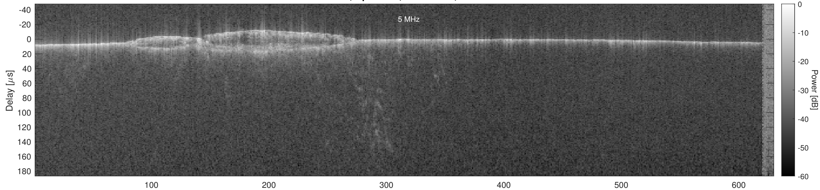
Orbit 7492, Optimized, No Window, Channel 2
