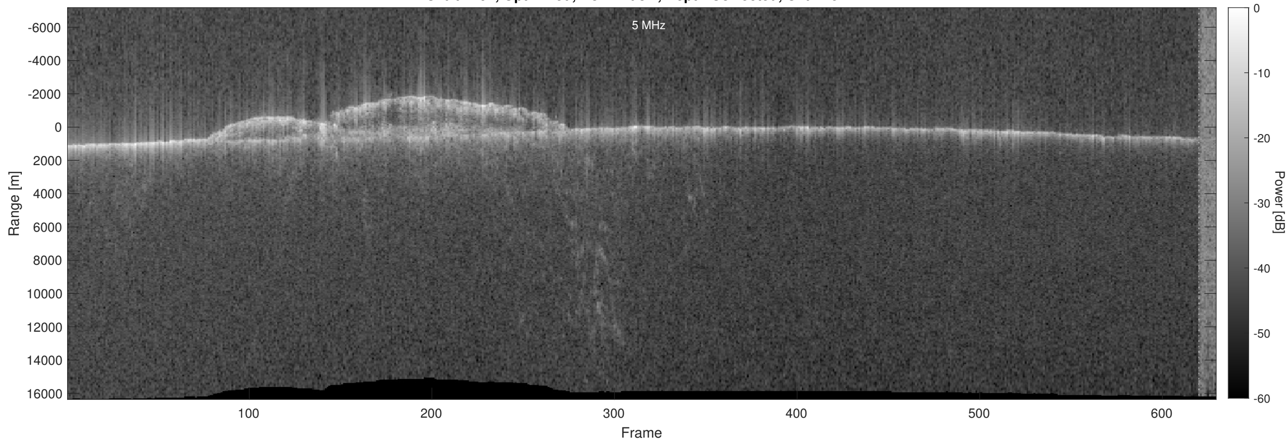
Orbit 7492, Optimized, No Window, Depth-Corrected, Channel 2
