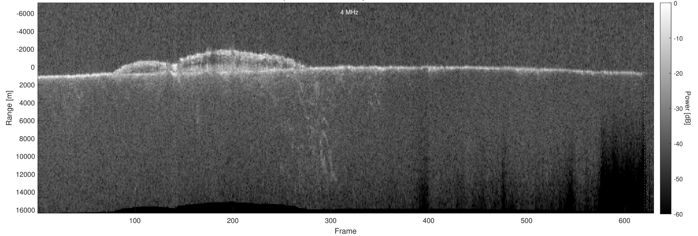
Orbit 7492, Optimized, Window, Depth-Corrected, Channel 2
