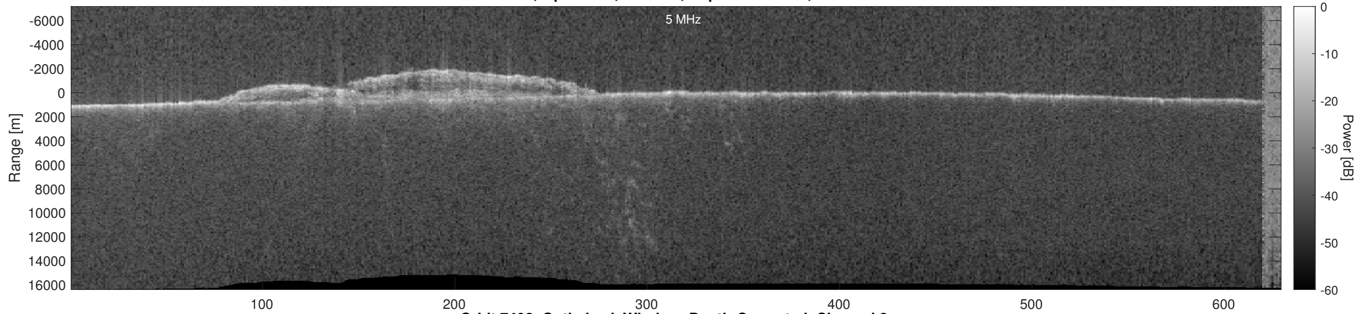
Orbit 7492, Optimized, Window, Depth-Corrected, Channel 2
