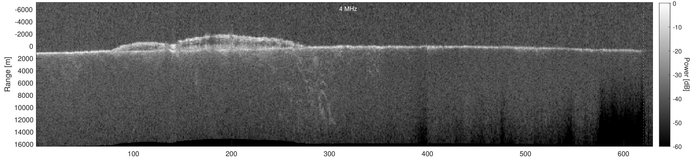
Orbit 7492, Depth-Corrected Cluttergram
