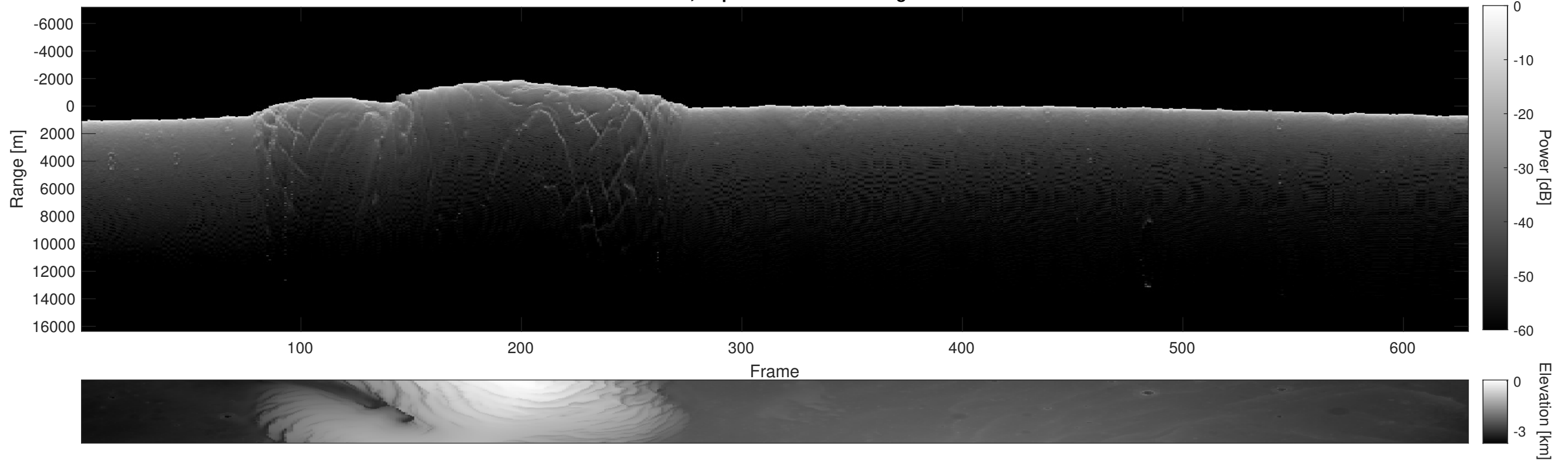
Orbit 7492, Depth-Corrected Cluttergram
