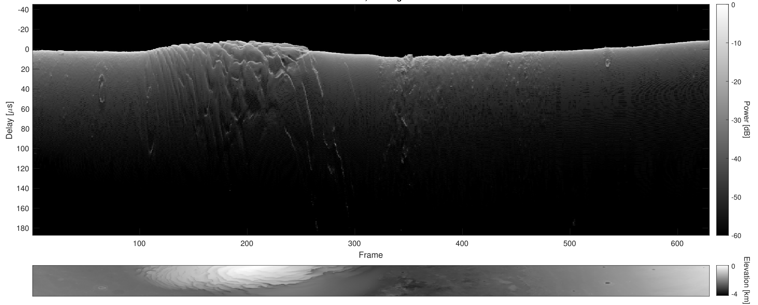
Orbit 7498, Cluttergram
