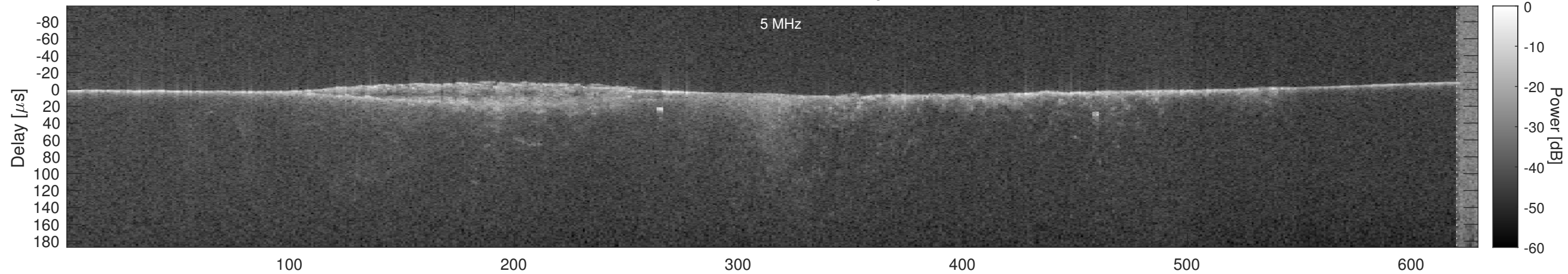
Orbit 7498, Cluttergram
