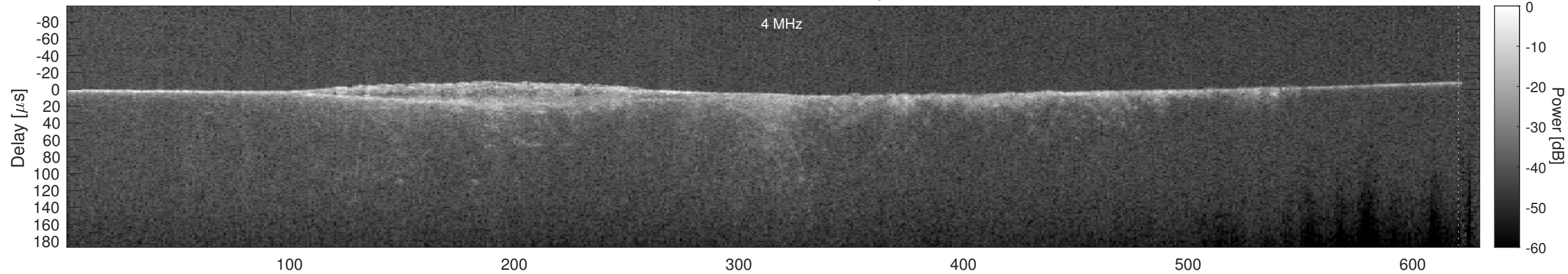
Orbit 7498, Cluttergram
