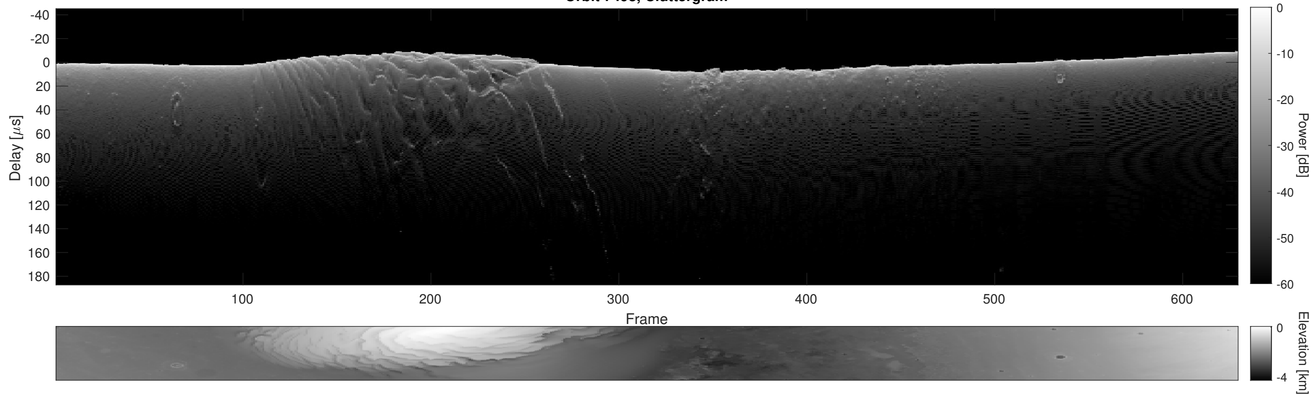
Orbit 7498, Cluttergram
