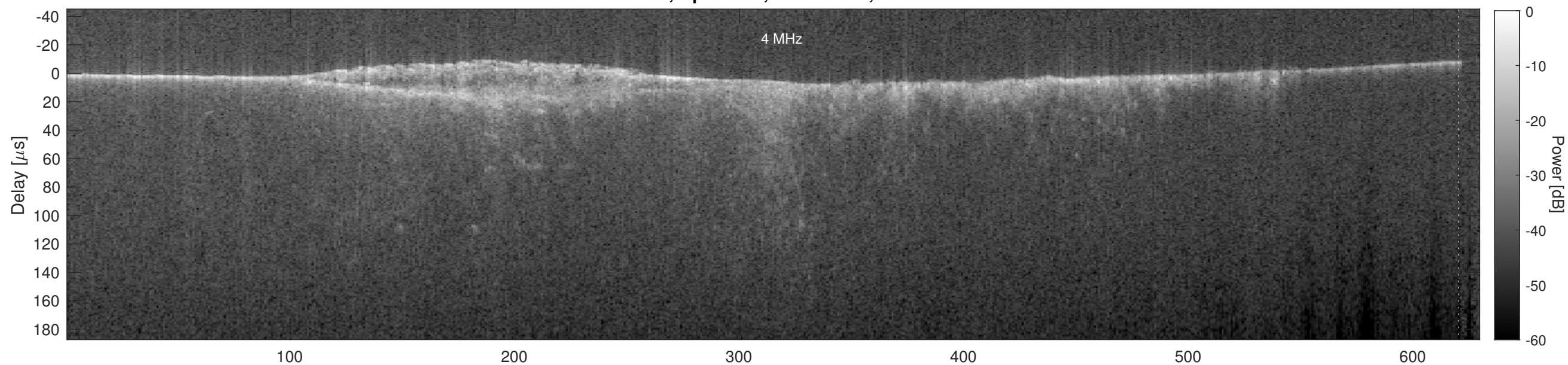
Orbit 7498, Cluttergram
