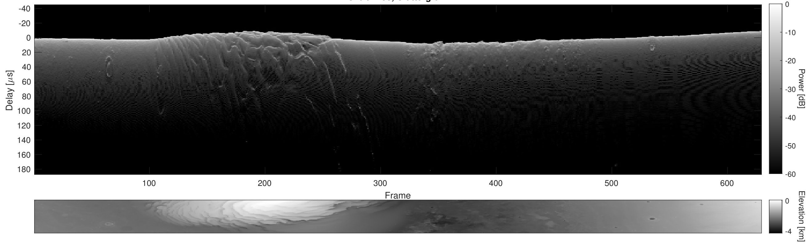
Orbit 7498, Cluttergram
