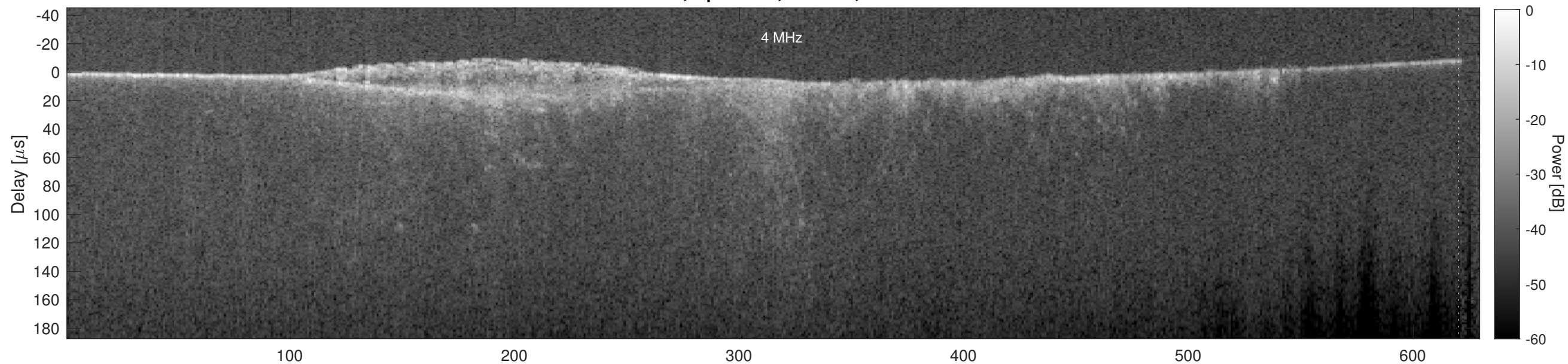
Orbit 7498, Cluttergram
