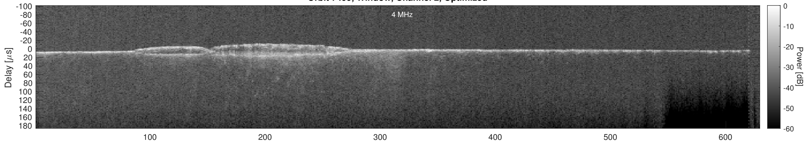
Orbit 7499, Cluttergram
