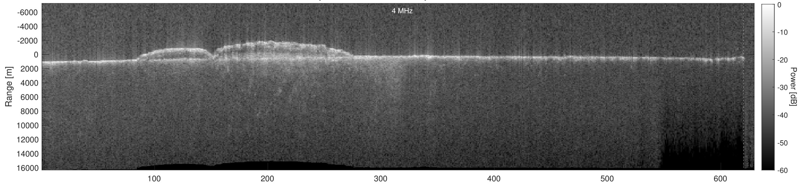
Orbit 7499, Depth-Corrected Cluttergram
