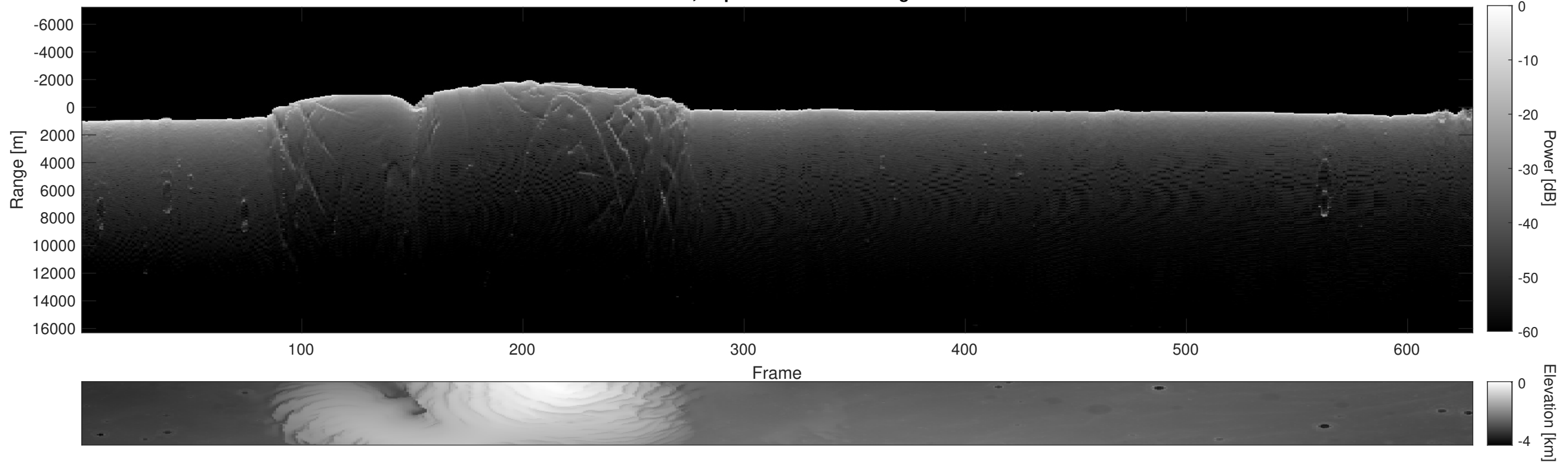
Orbit 7499, Depth-Corrected Cluttergram
