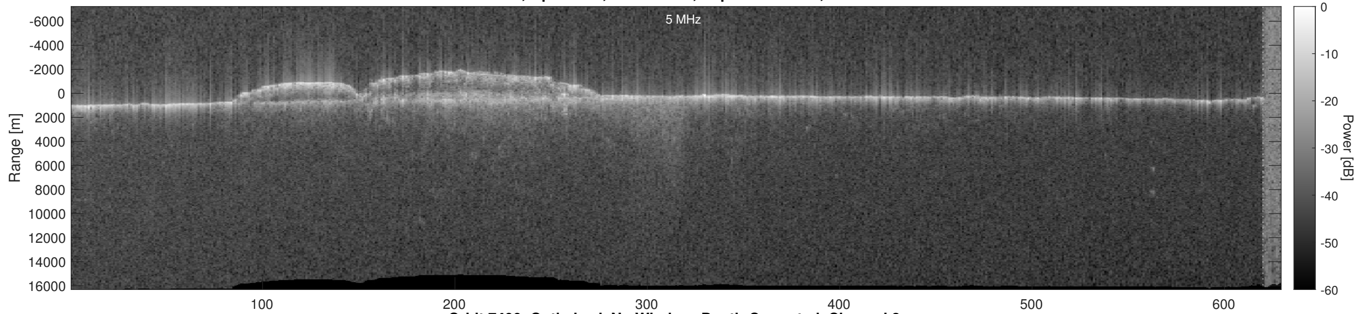
Orbit 7499, Optimized, No Window, Depth-Corrected, Channel 2
