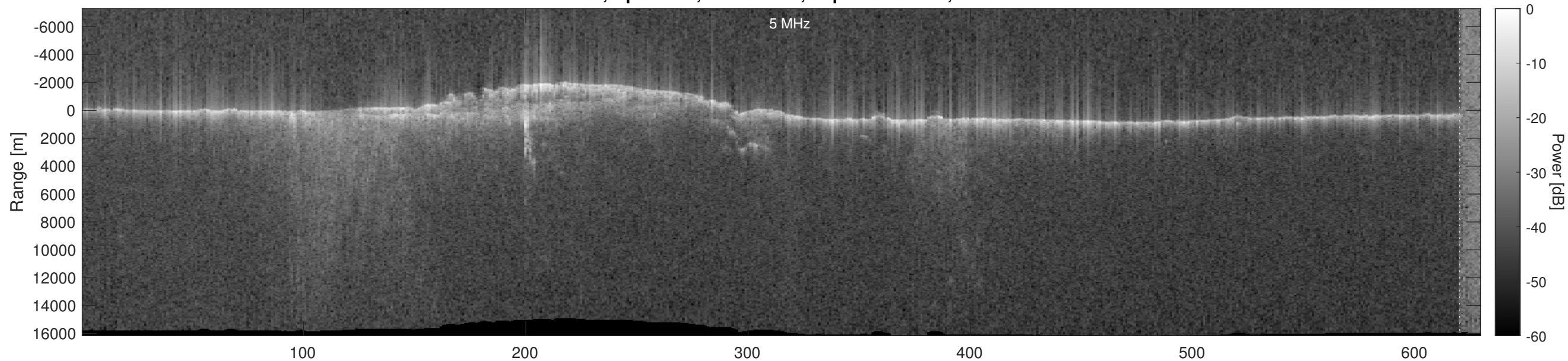
Orbit 7501, Optimized, No Window, Depth-Corrected, Channel 2
