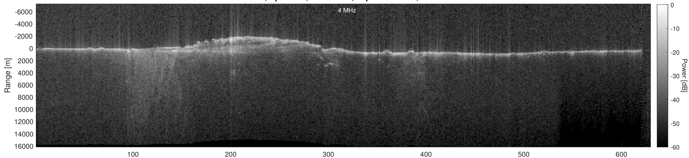
Orbit 7501, Depth-Corrected Cluttergram
