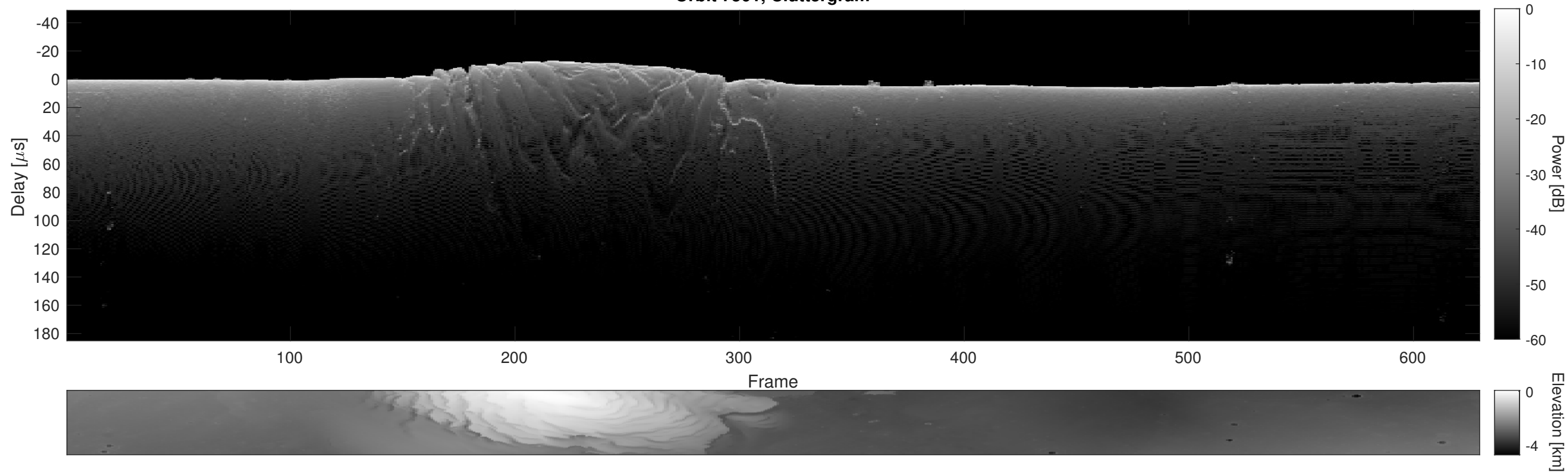
Orbit 7501, Cluttergram
