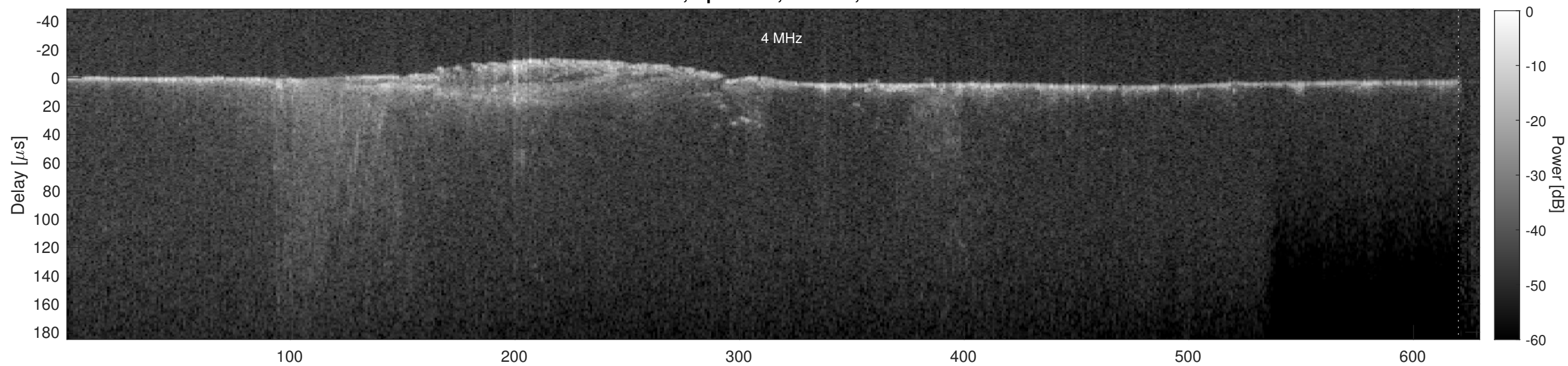
Orbit 7501, Cluttergram
