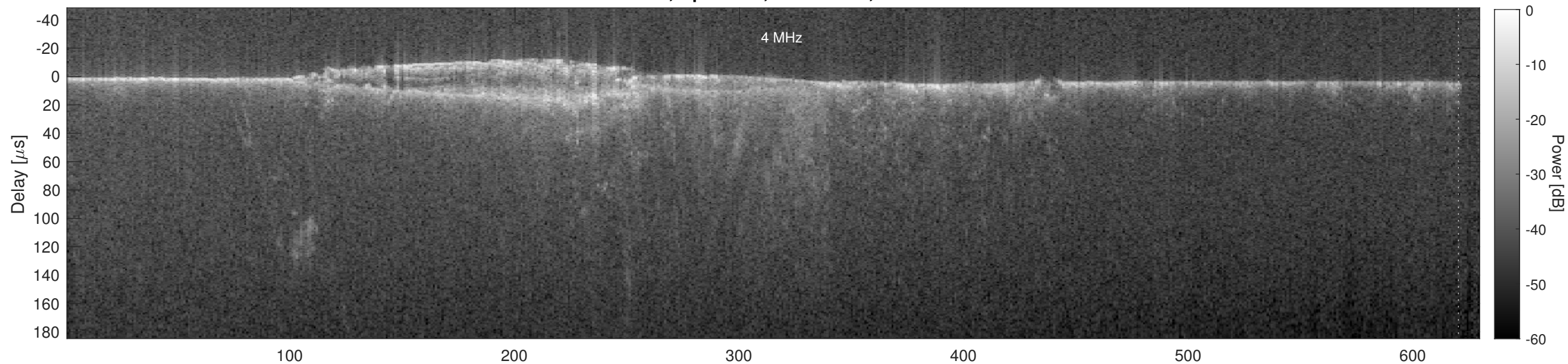
Orbit 7502, Cluttergram
