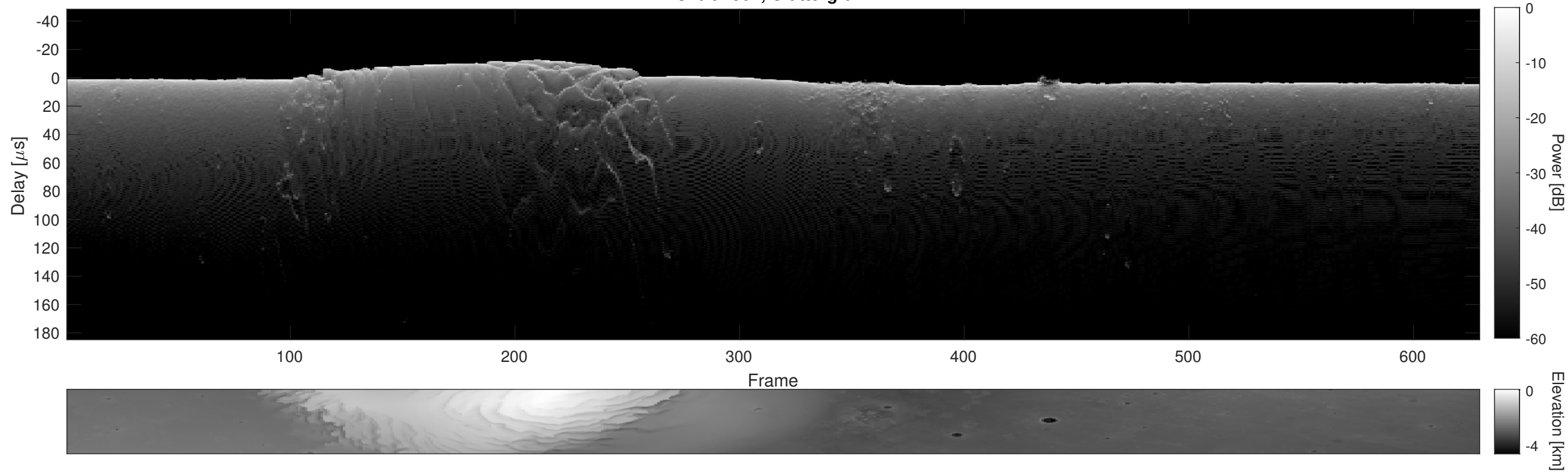
Orbit 7502, Cluttergram
