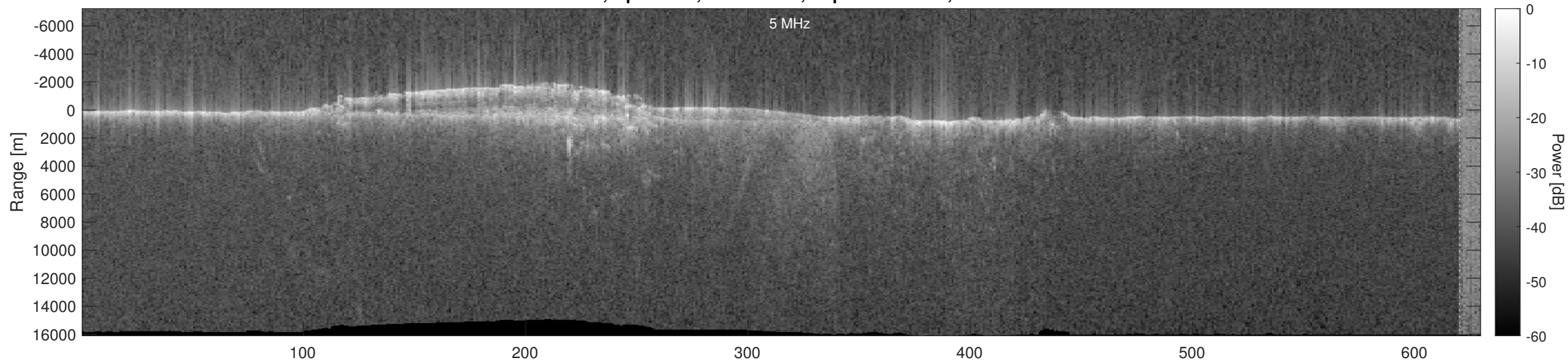
Orbit 7502, Optimized, No Window, Depth-Corrected, Channel 2
