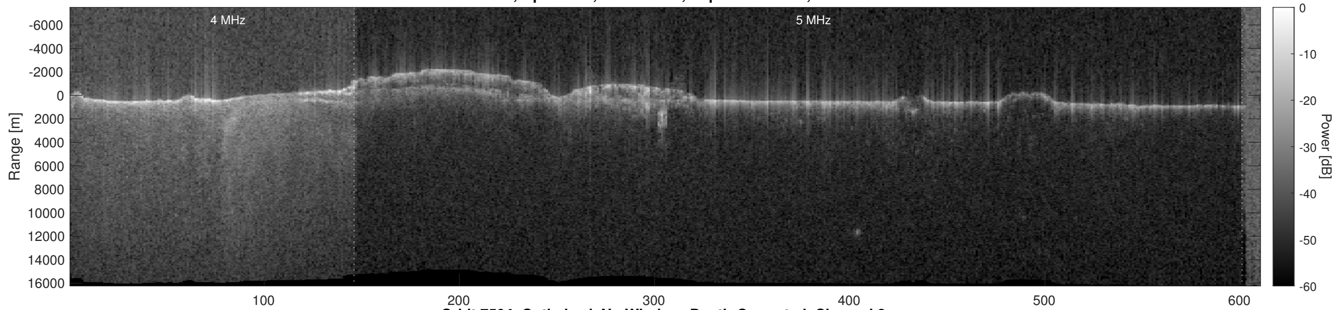
Orbit 7504, Optimized, No Window, Depth-Corrected, Channel 2
