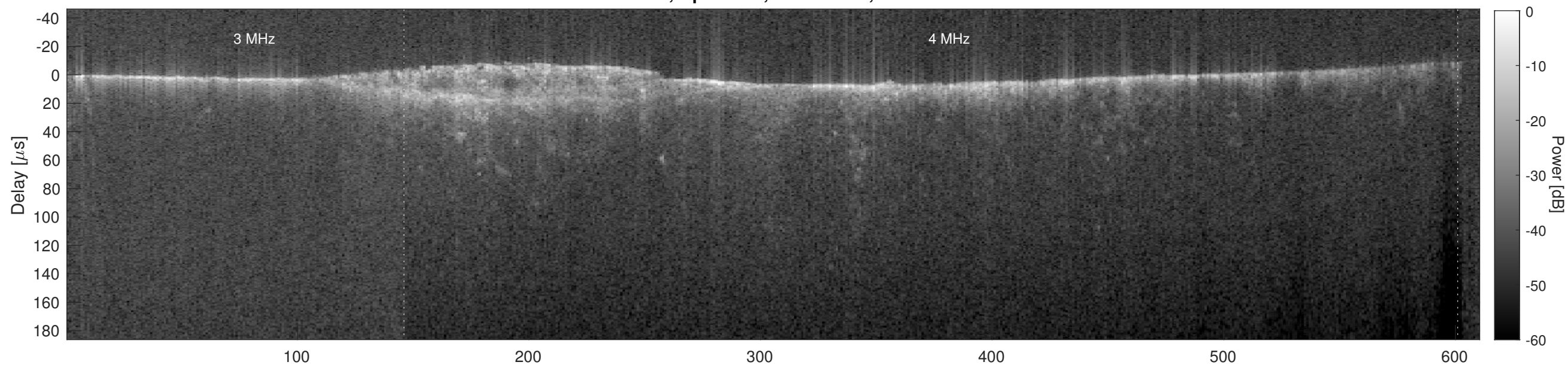
Orbit 7505, Cluttergram
