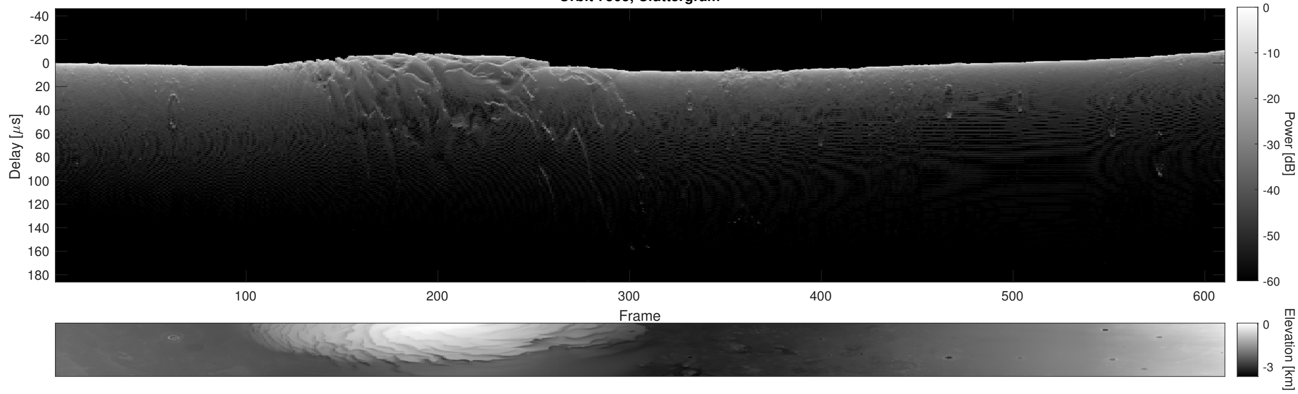
Orbit 7505, Cluttergram
