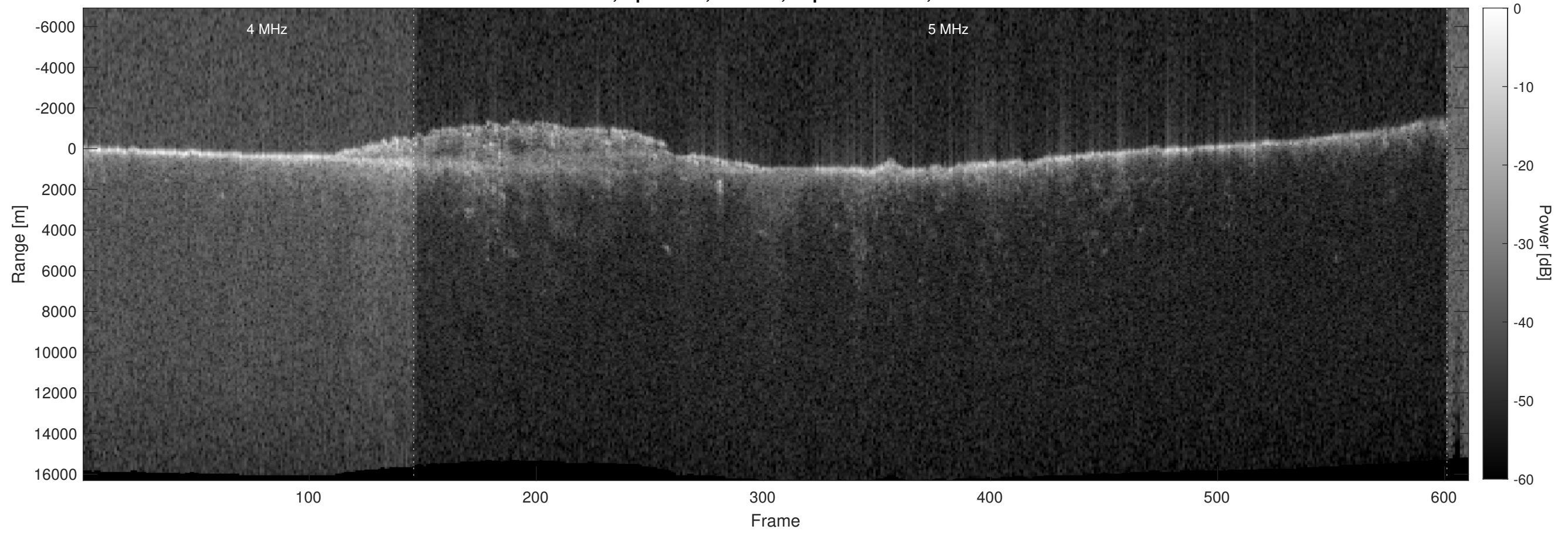
Orbit 7505, Optimized, Window, Depth-Corrected, Channel 2
