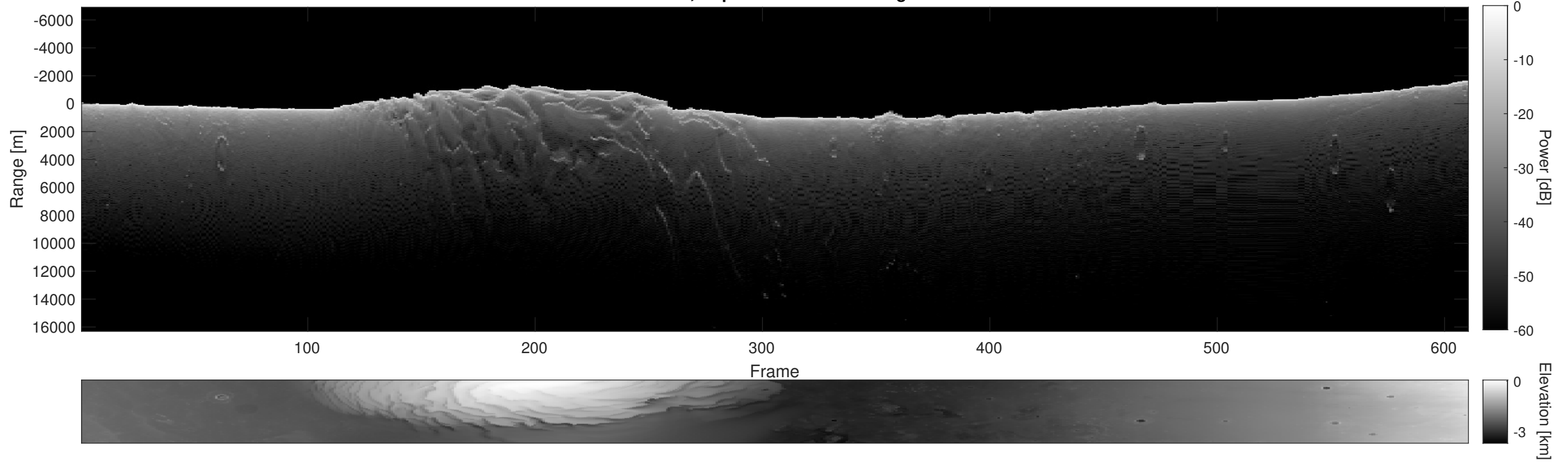
Orbit 7505, Depth-Corrected Cluttergram
