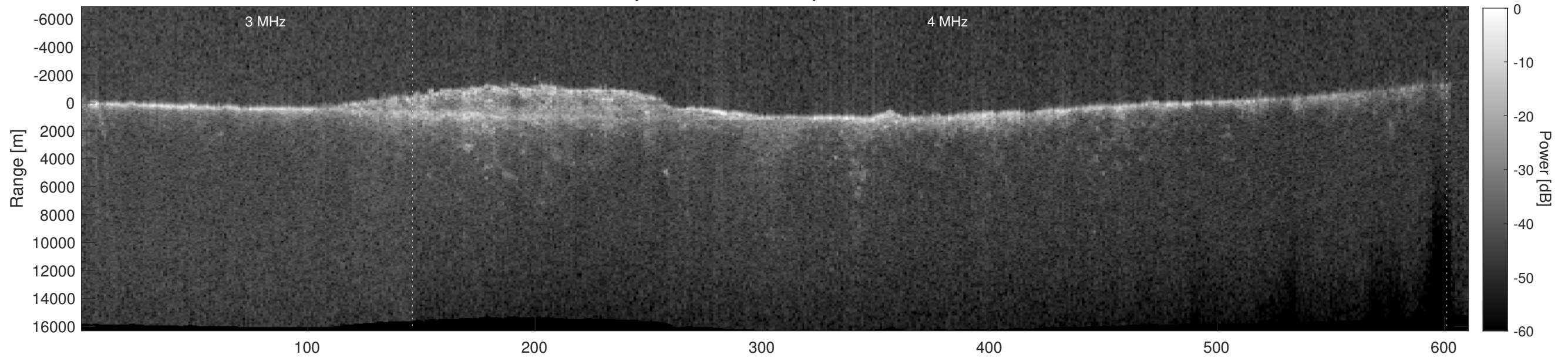
Orbit 7505, Depth-Corrected Cluttergram
