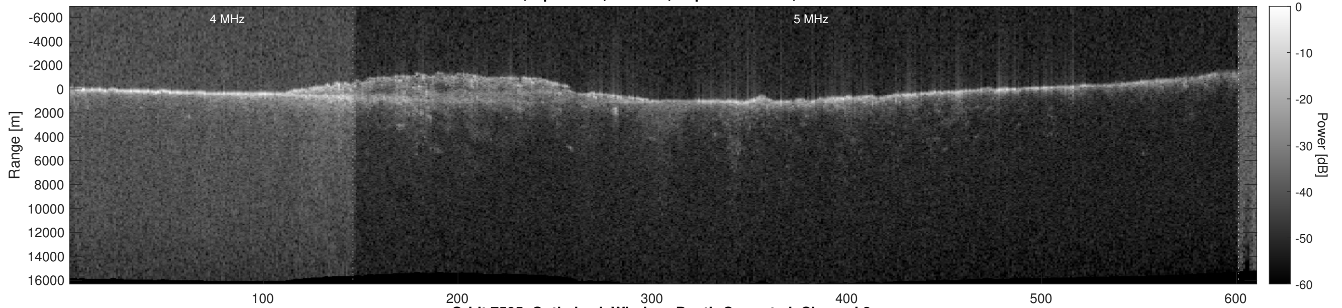
Orbit 7505, Optimized, Window, Depth-Corrected, Channel 2
