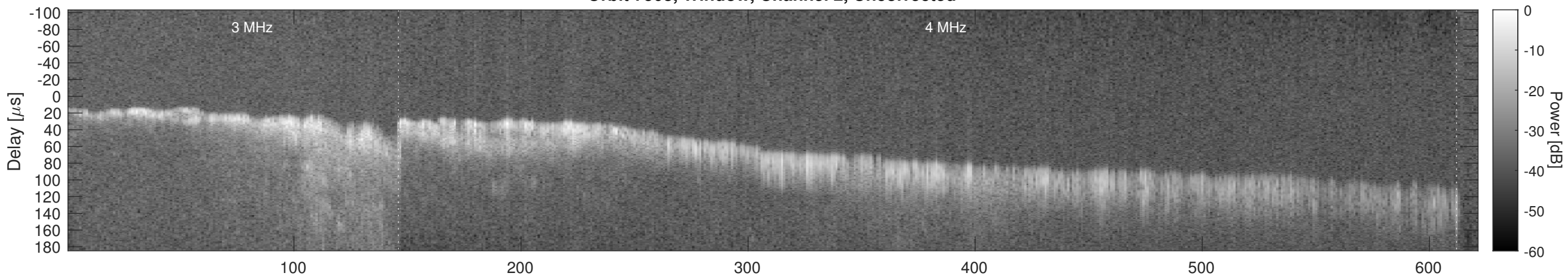
Orbit 7508, Window, Channel 2, Chapman
