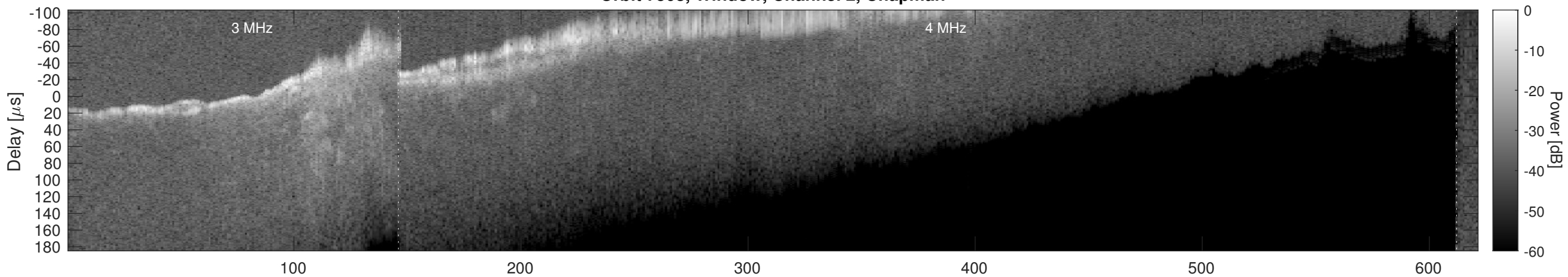
Orbit 7508, Window, Channel 2, Optimized
