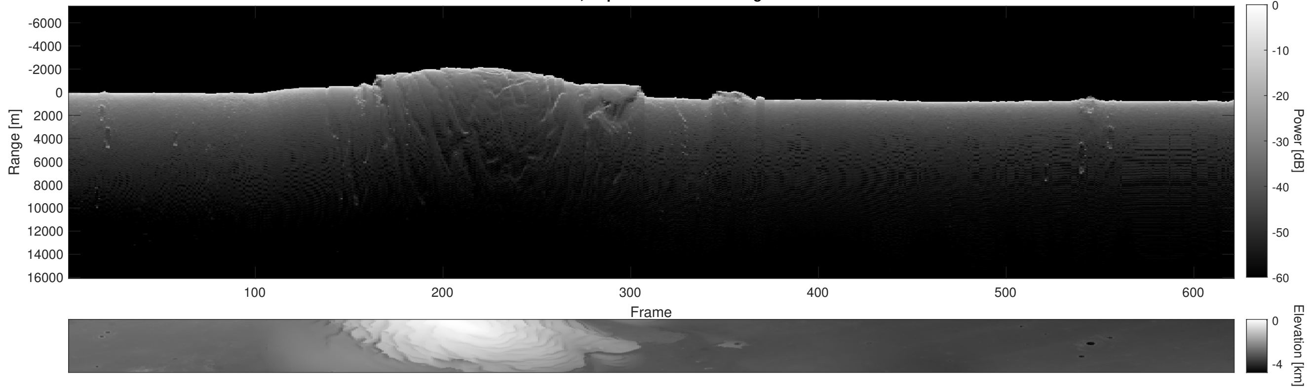
Orbit 7508, Depth-Corrected Cluttergram
