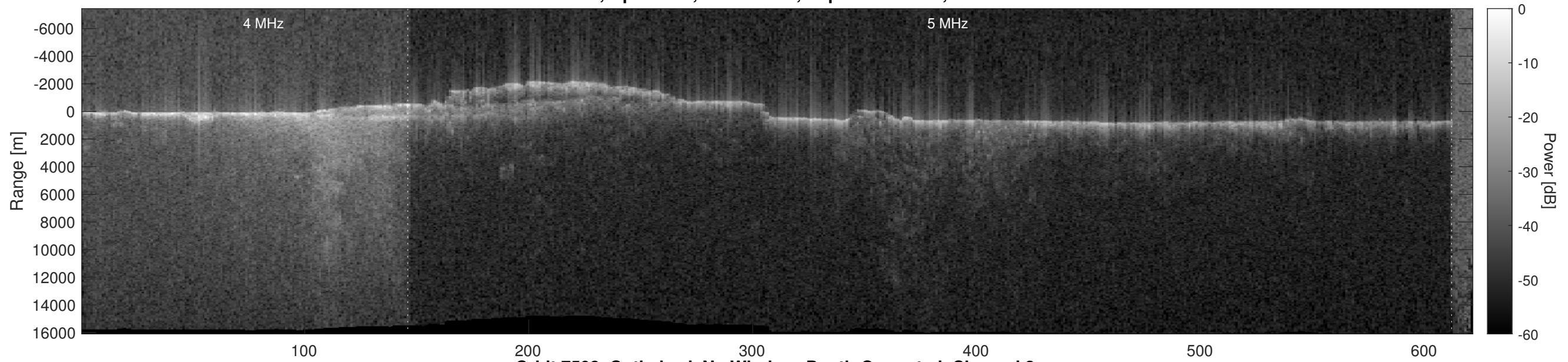
Orbit 7508, Optimized, No Window, Depth-Corrected, Channel 2
