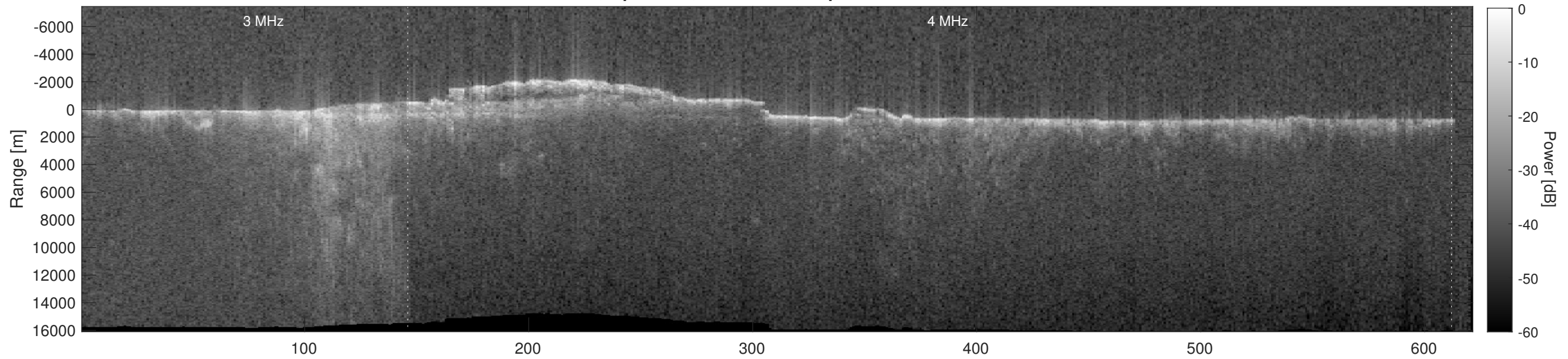
Orbit 7508, Depth-Corrected Cluttergram
